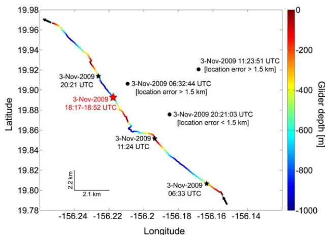
Figure 5. Glider track (colored line) and surfacing positions of tagged Cuvier's beaked whale (black dots) on 3 November 2009. Glider depth is color-coded. Black stars indicate position of glider at times of beaked whale surfacing events. Red star indicates position of glider when Cuvier's beaked whale clicks were acoustically detected by the glider during the mission (detections were verified in the post deployment analysis). The acoustic system was operated at depth between 500 m and 1000 m indicated by greenish/bluish colors. Times are UTC.
