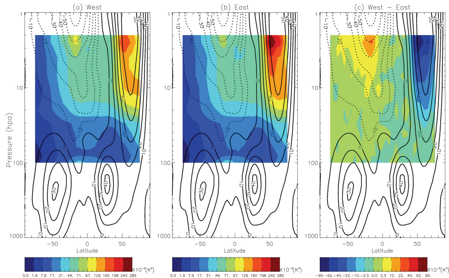
Fig. 3. Zonal mean of the GW variance at the westmost view (a) , eastmost view (b) and the difference between the westmost and eastmost views (c) as a function of latitude and height for January, 2005. Monthly mean zonal winds obtained from UK Met Office are contoured in solid (westerly) and dotted (easterly) lines with an interval of 10 \text{ m s}^{-1} . The color scale is linear by taking a square-root of the values. In (c) , positive (negative) values correspond to preferred eastward (westward) propagation direction.
