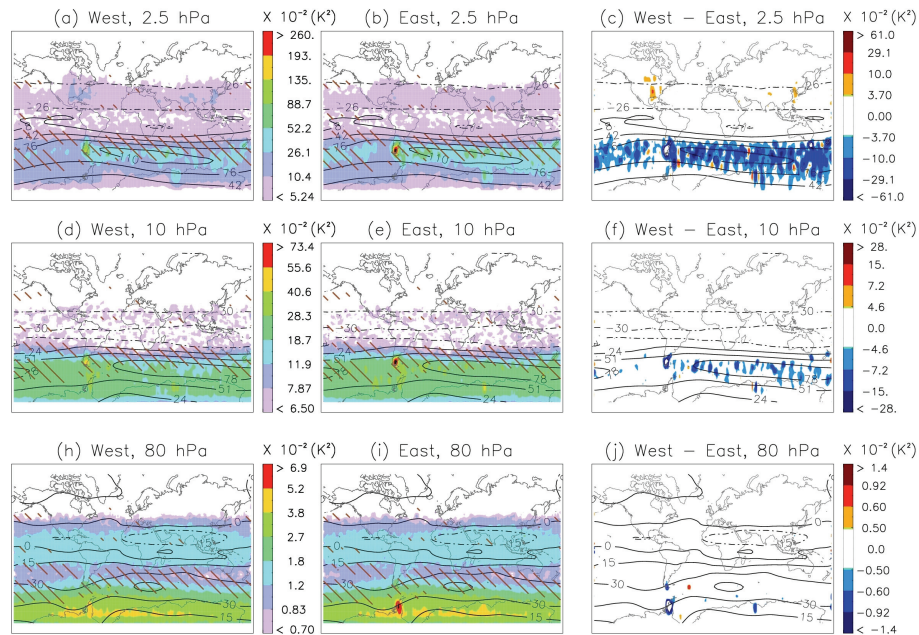
Fig. 6. Same as Fig. 5, except for July 2005.
