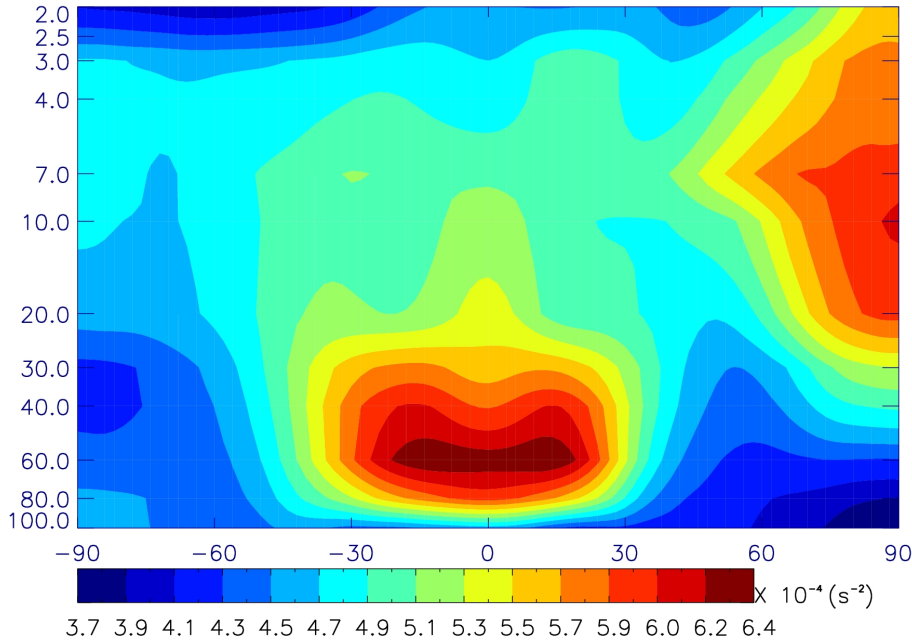
Fig. B1. Zonal mean of the Brunt-Väisälä frequency ( N^2 ) as a function of latitude and height for January 2005, derived from ERA Interim dataset.
