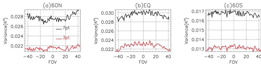
Fig. 10. Zonal mean FOV curves at 80 hPa for 3-pt (red) and 7-pt (black) results at January 2005 at 60° N (a) , 0° (b) and 60° S (c) . The horizontal axes are the number of scanning points along a FOV scan, where -(+) 45 corresponds to westmost(eastmost) view, while 0 is at nadir.
