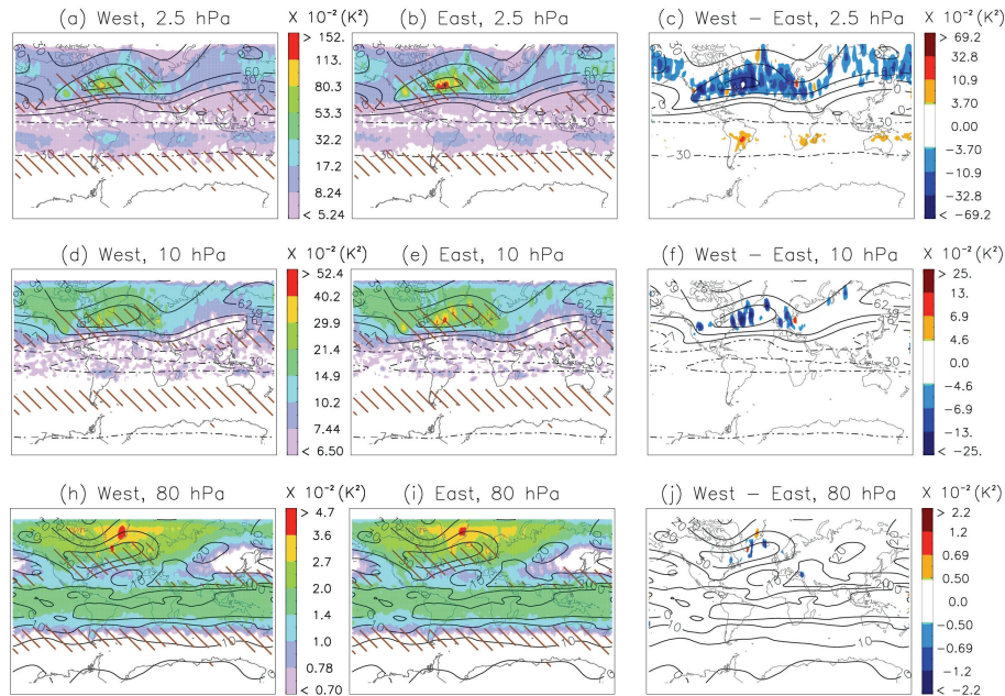
Fig. 5. Geographical distribution of GW variance on a 2^\circ \times 2^\circ grid at westmost view (left column), eastmost view (middle column) and the difference (right column) for January 2005 at 2.5, 10, and 80 hPa from top to bottom. 3-pt smoothing has been further applied to make the signals stand out. In the left two columns, values smaller than 2\sigma are uncolored, where \sigma is the minimum detectable variance. In the rightmost column, absolute values smaller than \sqrt{2}\sigma are whitened, where \sqrt{2}\sigma is the smallest detectable difference. The UK Met Office monthly mean zonal winds at corresponding levels are contoured in black solid (westward) and dotted (eastward) lines. Total wind velocity greater than 10 \text{ m s}^{-1} areas at 700 hPa are hatched with brown lines.
