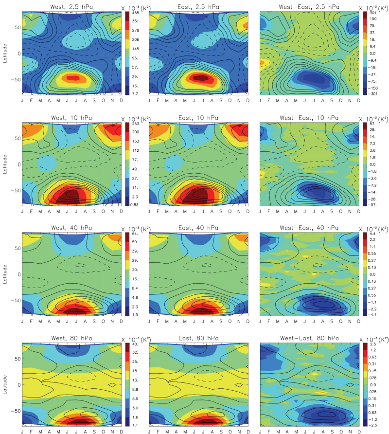
Fig. 7. Multi-year averaged timeseries of GW variance for different months at westmost view (first column), eastmost view (second column) and the difference (third column) at 2.5, 10, 40 and 80 hPa from top to bottom. The UK Met Office zonal winds are overplotted in solid (dashed) lines representing westerlies (easterlies) with contour interval of 10 \text{ m s}^{-1} .
