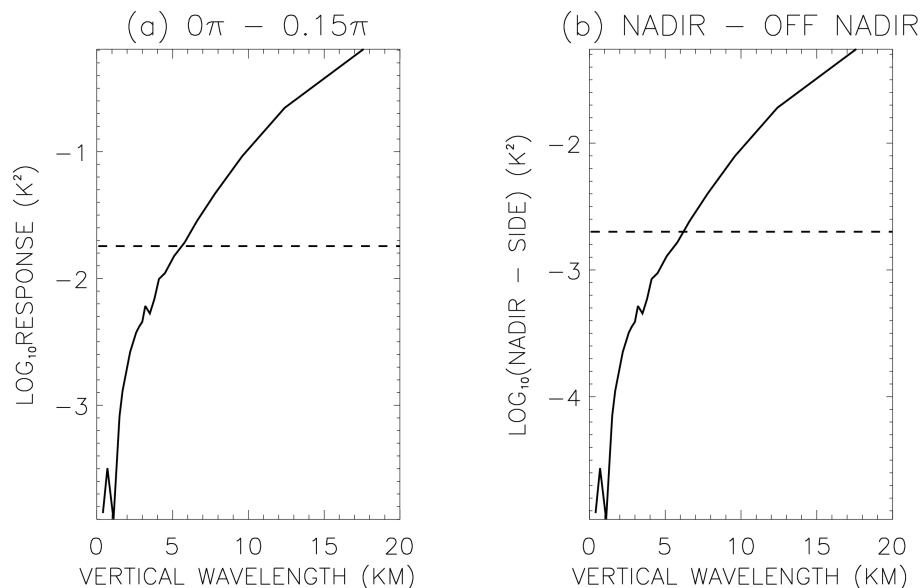
Fig. 12. Variance differences between unshifted wave and the wave shifted by 0.15\pi for \lambda_x = 700 km calculation (a) , and the variance difference between nadir FOV and the outmost FOV (b) as functions of \lambda_z . The AIRS observed values (7-pt smoothing window applied) are denoted by dash lines. See text for details.
