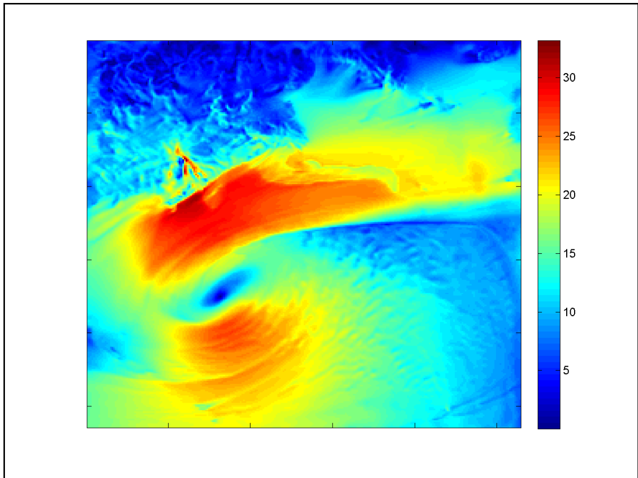
Figure 2. WRF surface wind speed ( \text{ms}^{-1} ) corresponding to the cyclone imaged in Figure 1 at 1700 UTC on 24 January 2008.
