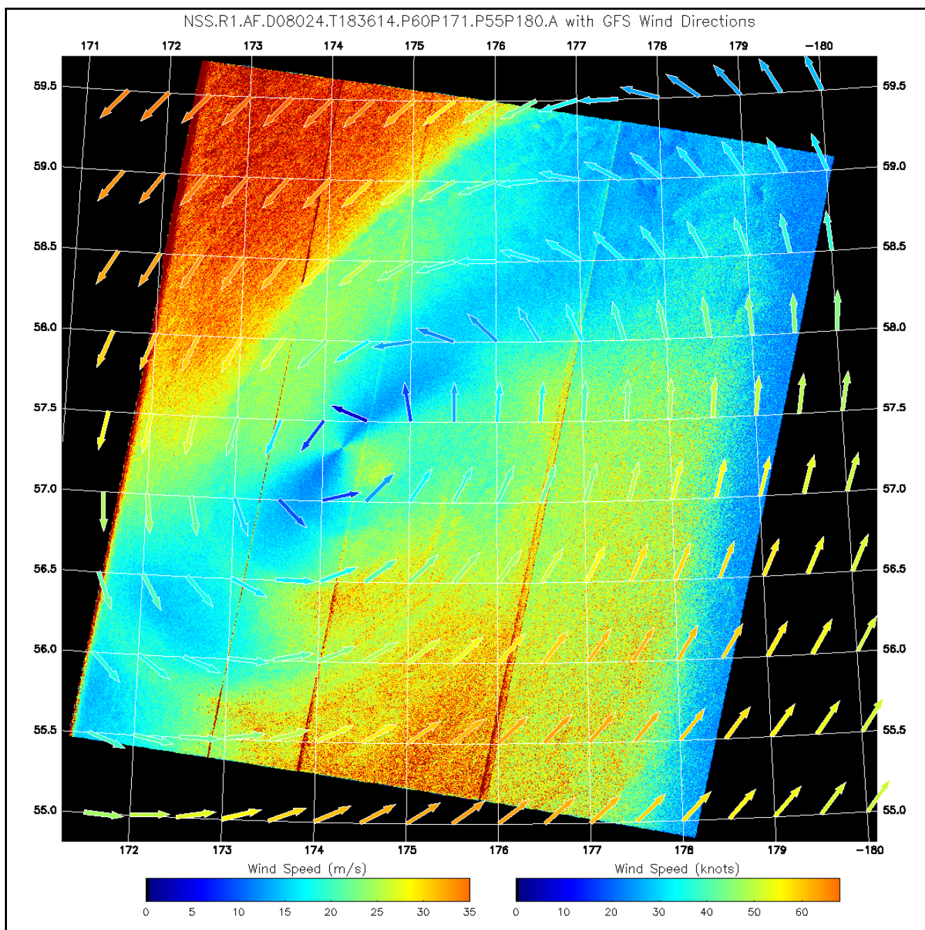
Figure 1. SDWS overlaid by GFS-analyzed surface wind vectors depict a conveyor belt of large wind speed spiraling into the center of a mature cyclone in the Bering Sea at 1836 UTC on 24 January 2008. (Provided courtesy of JHUAPL)
