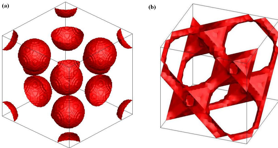
Figure 6. Iso-surface plots of dielectric permittivity (based upon equations) for (a) the discrete sphere model and (b) for the minimal surface model of the diamond configuration with 19% volume fraction
