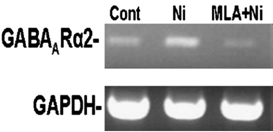
FIG E6. MLA blocks nicotine ( Ni )–induced GABA A R2α in A549 cells. mRNA from A549 cells after treatment with nicotine and nicotine plus MLA (1 μmol/L) was analyzed by using RT-PCR, as described in the Methods section.
