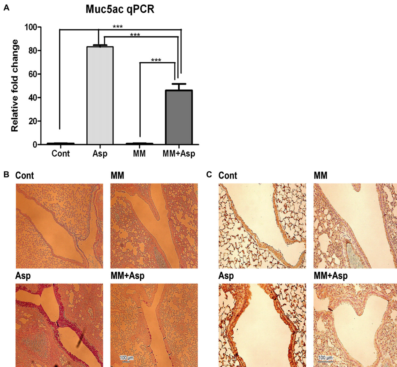
FIG 5. Aspergillus species induces MM-sensitive GABA A R \alpha 2 expression and mucus formation in the lung. BALB/c mice were sensitized with Aspergillus fumigatus (Asp) extracts and, where indicated, received MM. Lungs were tested for Muc5ac by using qPCR (A), mucus by using AB/PAS staining (B), and GABA A R \alpha 2 by using IHC (C). The results represent 2 independent experiments with 3 to 6 mice per group. *** P \leq .001 .
