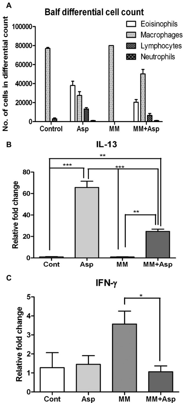
FIG E8. Aspergillus species ( Asp ) induce MM-sensitive GABA _A R \alpha 2 and mucus formation in the airways. BALB/c wild-type mice were exposed to Aspergillus fumigatus extract, as described in the Methods section. Some animals received the nAChR inhibitor MM. Differential cell counts in bronchoalveolar lavage fluid ( A ), lung IL-13 expression determined by using qPCR ( B ), and lung IFN- \gamma expression determined by using qPCR in various groups ( C ) are shown. The results represent 2 independent in vivo exposure experiments with 3 to 6 mice per group. * P \leq .05 , ** P \leq .01 , and *** P \leq .001 .
