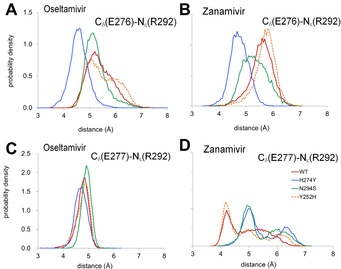
Figure 3. Comparison of WT and mutant dynamics. For WT and H274Y, N294S, and Y252H, distance distributions between the atoms C _{\delta} of E276 and N _{\epsilon} of R292 and between the atoms C _{\delta} of E277 and N _{\epsilon} of R292 are shown for oseltamivir (A, C) and zanamivir (B, D), respectively. doi:10.1371/journal.pcbi.1002665.g003
