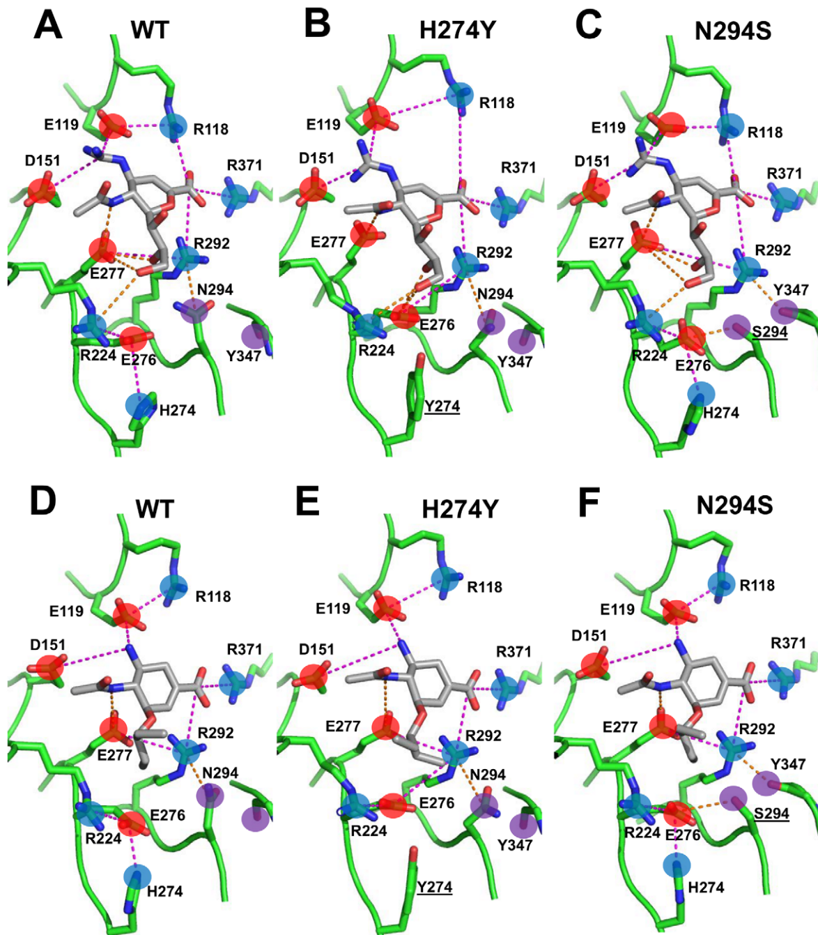
Figure 2. Representative structures for zanamivir (A, B and C) and oseltamivir (D, E and F) bound to WT and mutant NAs from the SRSN/HREX simulations. Salt-bridges and hydrogen bonds are depicted as magenta and orange dashed lines, respectively. Positively charged, negatively charged, and uncharged polar groups are noted as blue, red, and purple circles, respectively, and residues of interest are labeled. Mutated residues are underlined.
