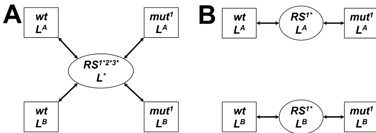
Figure 1. Alchemical thermodynamic paths using SRMM (A) and SRS (B) in the bound state between wild type (wt) and a mutant (mut¹). The paths (arrows) between end states (squares) going through nonphysical reference states (ovals) are shown. The SRMM uses a common reference state ‘hub’ for all mutations and ligands (RS 1*2*3* L * ); SRS uses a mutation and ligand-specific reference state (RS 1* L A ). Decoupled residues and ligands are noted by an ‘*’. Thermodynamic paths in the unbound state have a similar form but without the ligand.
