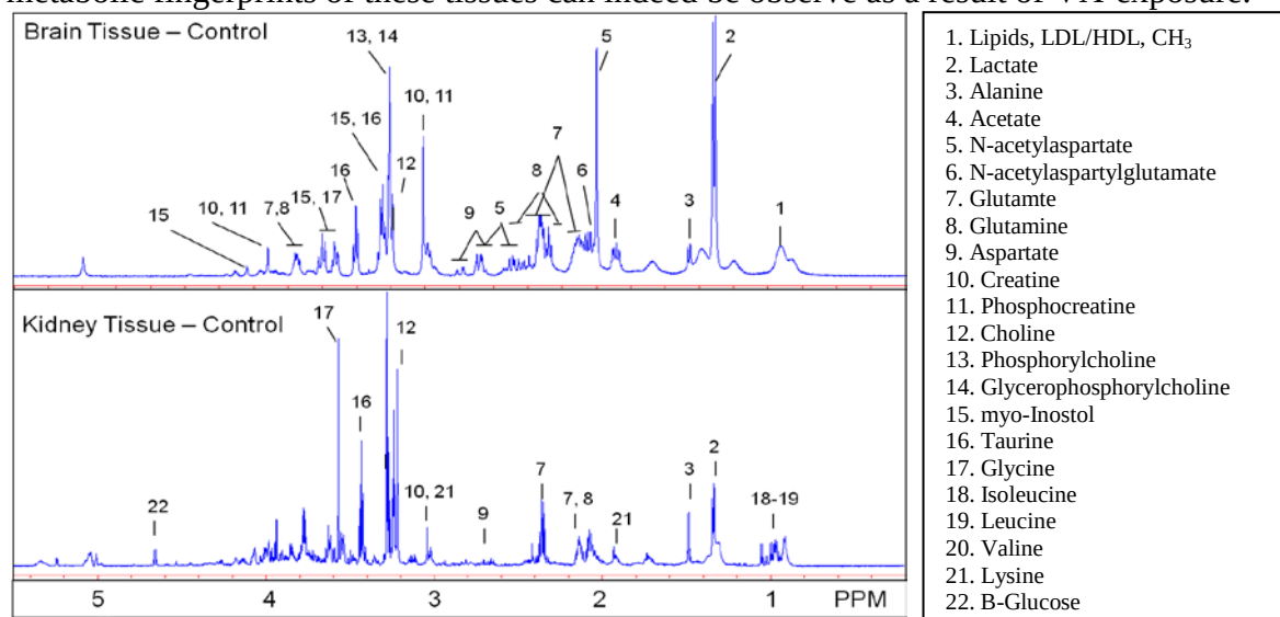
Figure 4: Expanded regions of ^1\text{H} CPMG spectra for rat brain tissue (top, 2ms total spin relaxation delay, 500 MHz) and for rat kidney tissue (bottom, 120 ms total spin-relaxation delay, 750 MHz). The assignments of selected metabolites are based on literature values. 18,19 The broad peaks in the brain tissue spectrum in the 0.7 to 1.4 ppm region are due to lipid that have not been completely edited out by the short CPMG relaxation delay.
