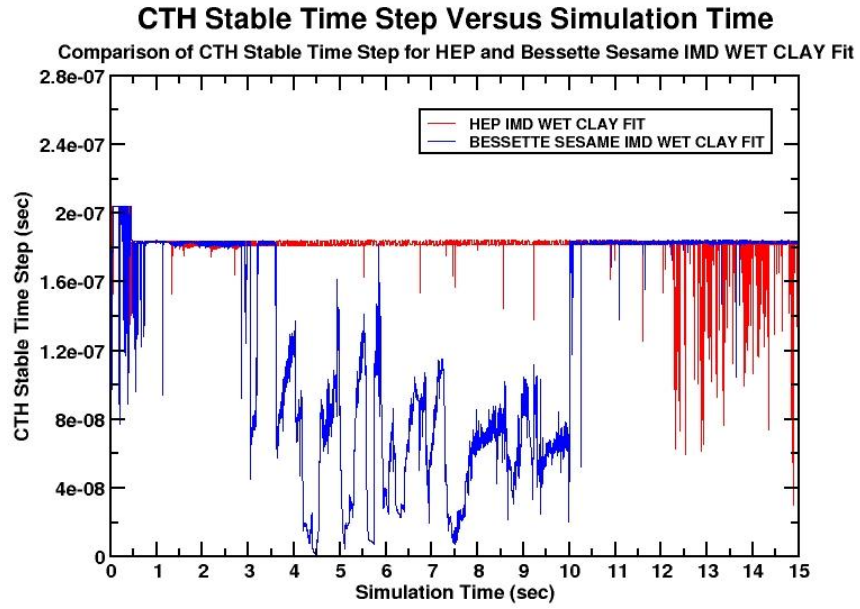
Figure 2. 26: Comparison of stable time step for HEP and Bessette WET CLAY runs
