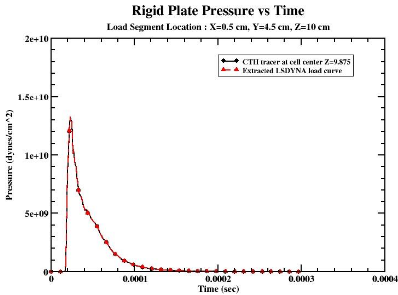
3.5a) Pressures at X=0.5, Y=4.5
