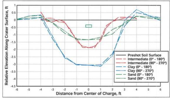
Figure 2. 15: Experimental crater dimensions (Ref. 20)
