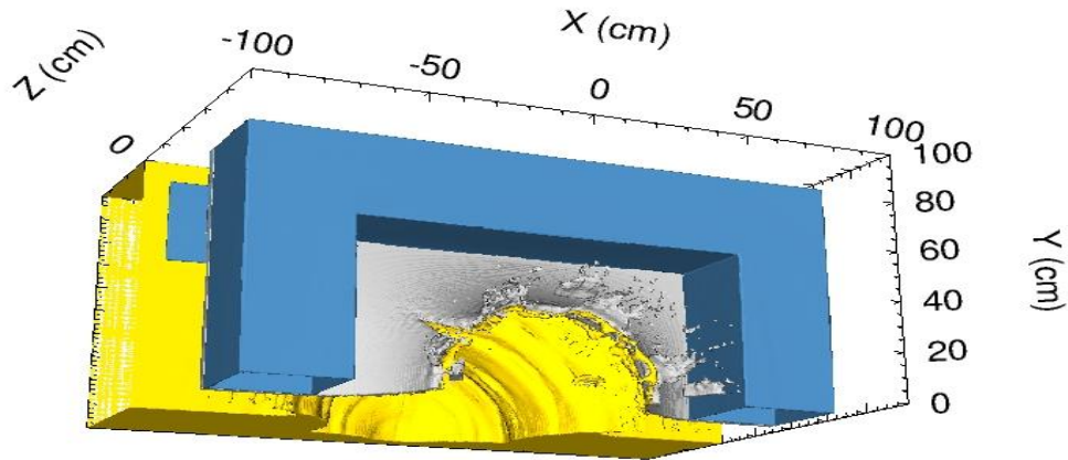
Figure 3. 15: DRDC plate deformation for CTH HEP analysis with default JC fracture values
