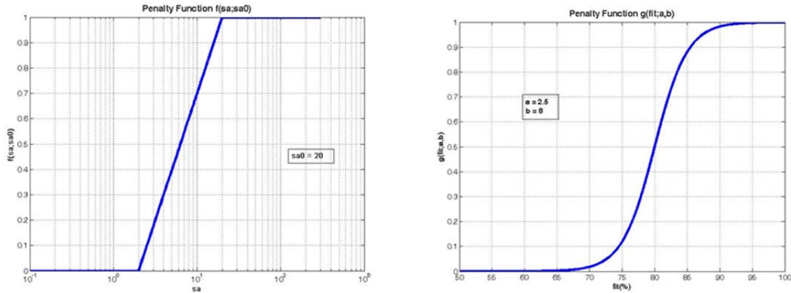
Figure 12. Data Confidence Penalty Sub-Functions f and g
