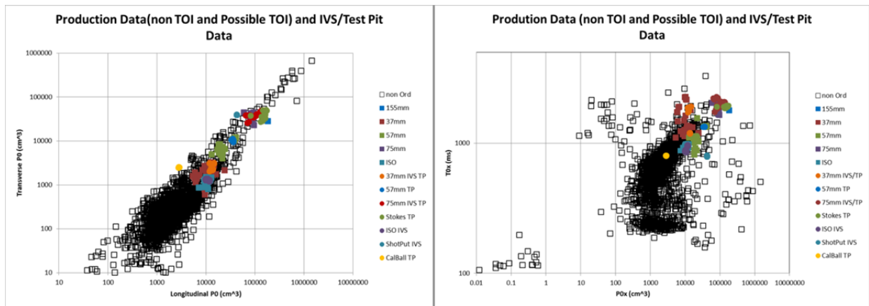
Figure 14. Distribution of PMTMA Data (Possible Ordnance Based on Interpretation From Polarizability Curves)
