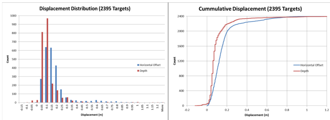
Figure 10. PMTMA Cued Production Data Displacement Statistics (Horizontal Offset and Depth)
