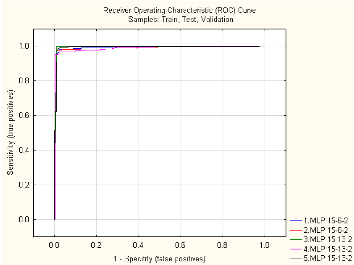
Figure 15. Five Best Trained ANN ROC Results
