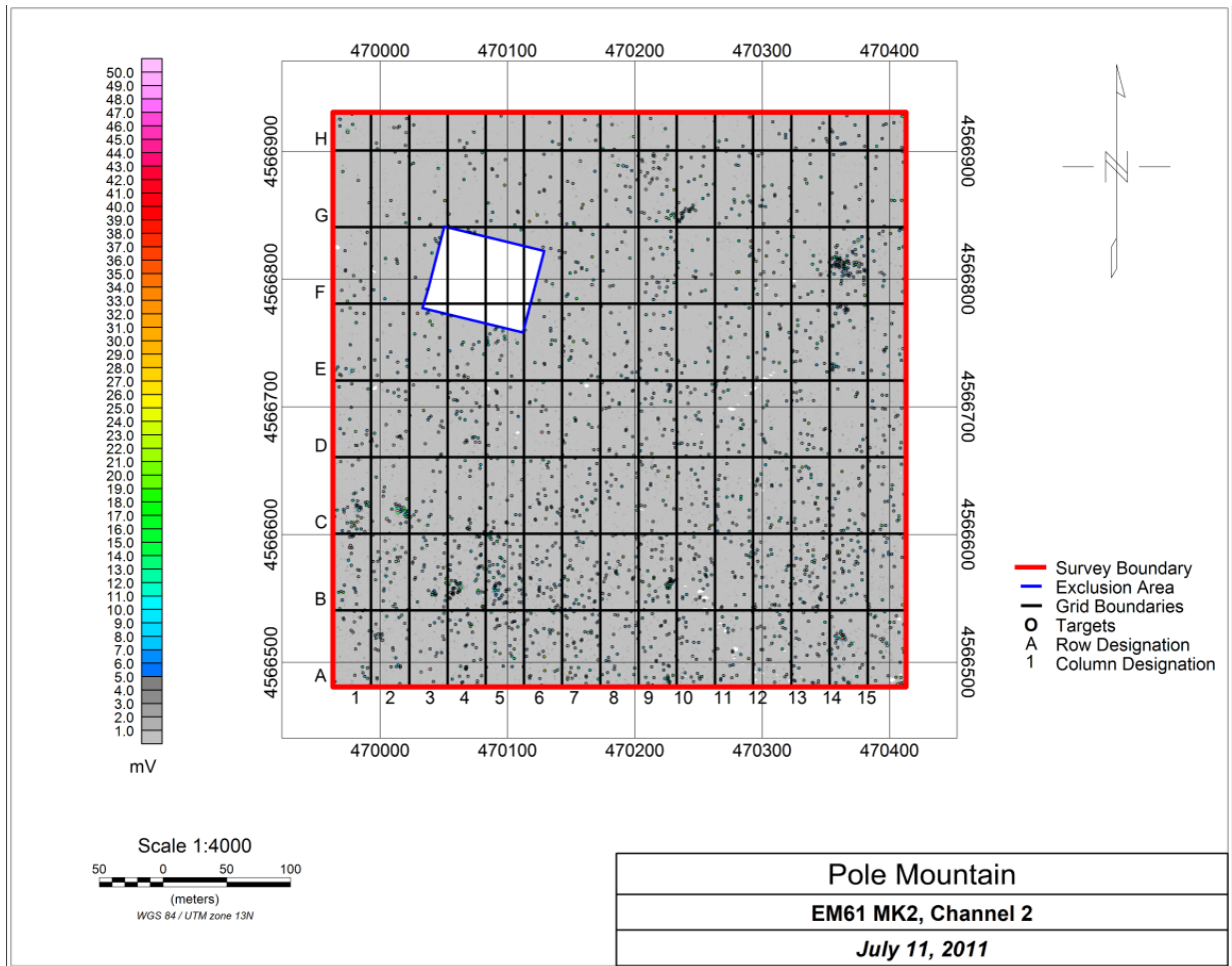
Figure 6. PMTMA EM61-MK2 Production Data with 2,370 Selected Targets and Grid Frame
