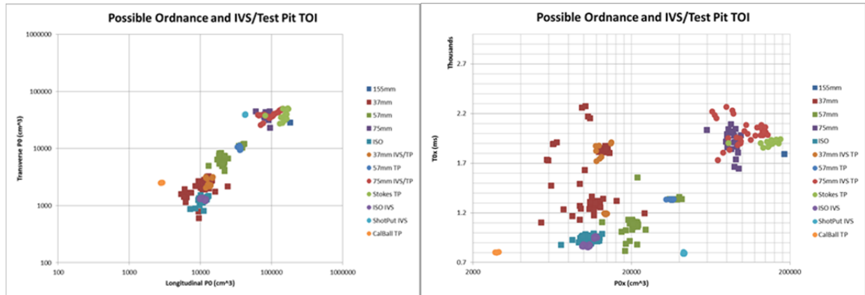
Figure 13. Distribution of Possible Ordnance (Interpretation From Polarizability Curves) and IVS/Test Pit Data for PMTMA Data
