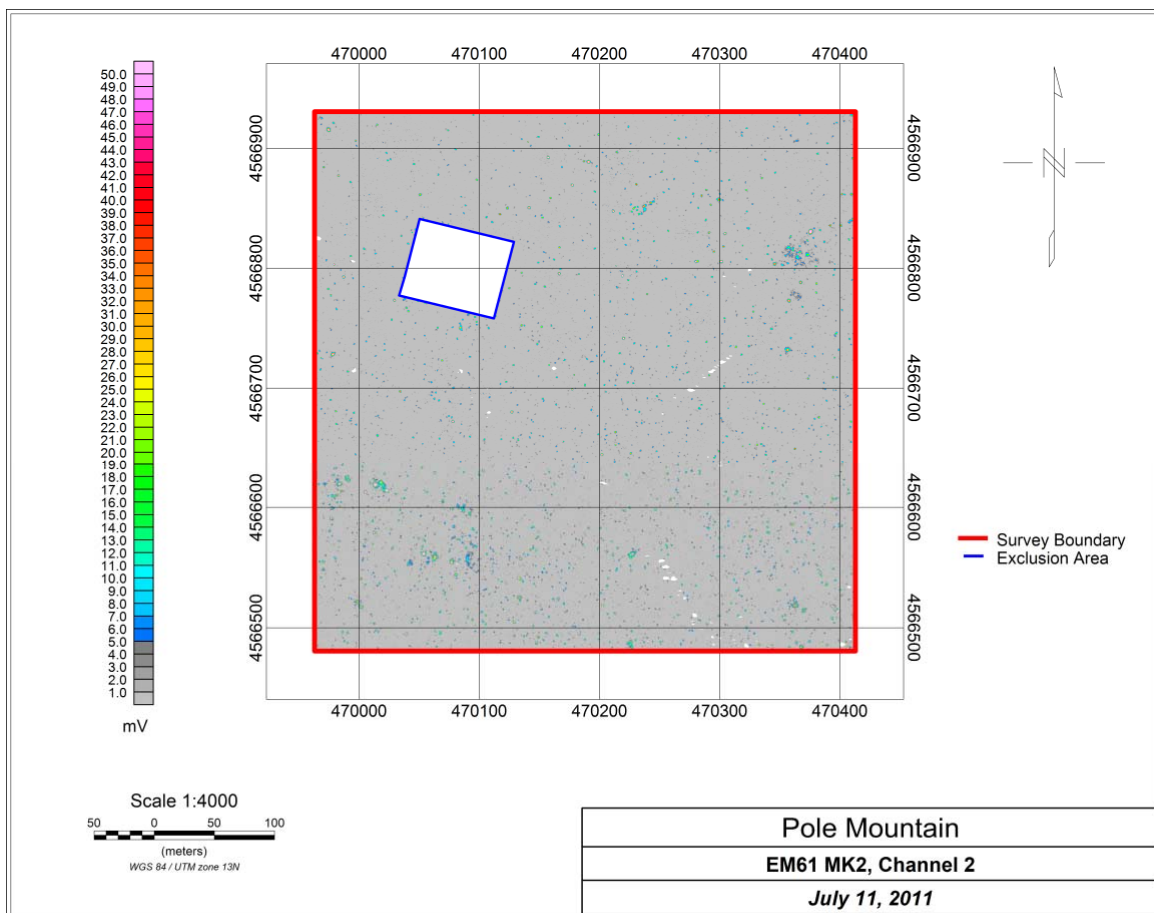
Figure 5. PMTMA EM61-MK2 Production Data Channel 2 Survey Results
