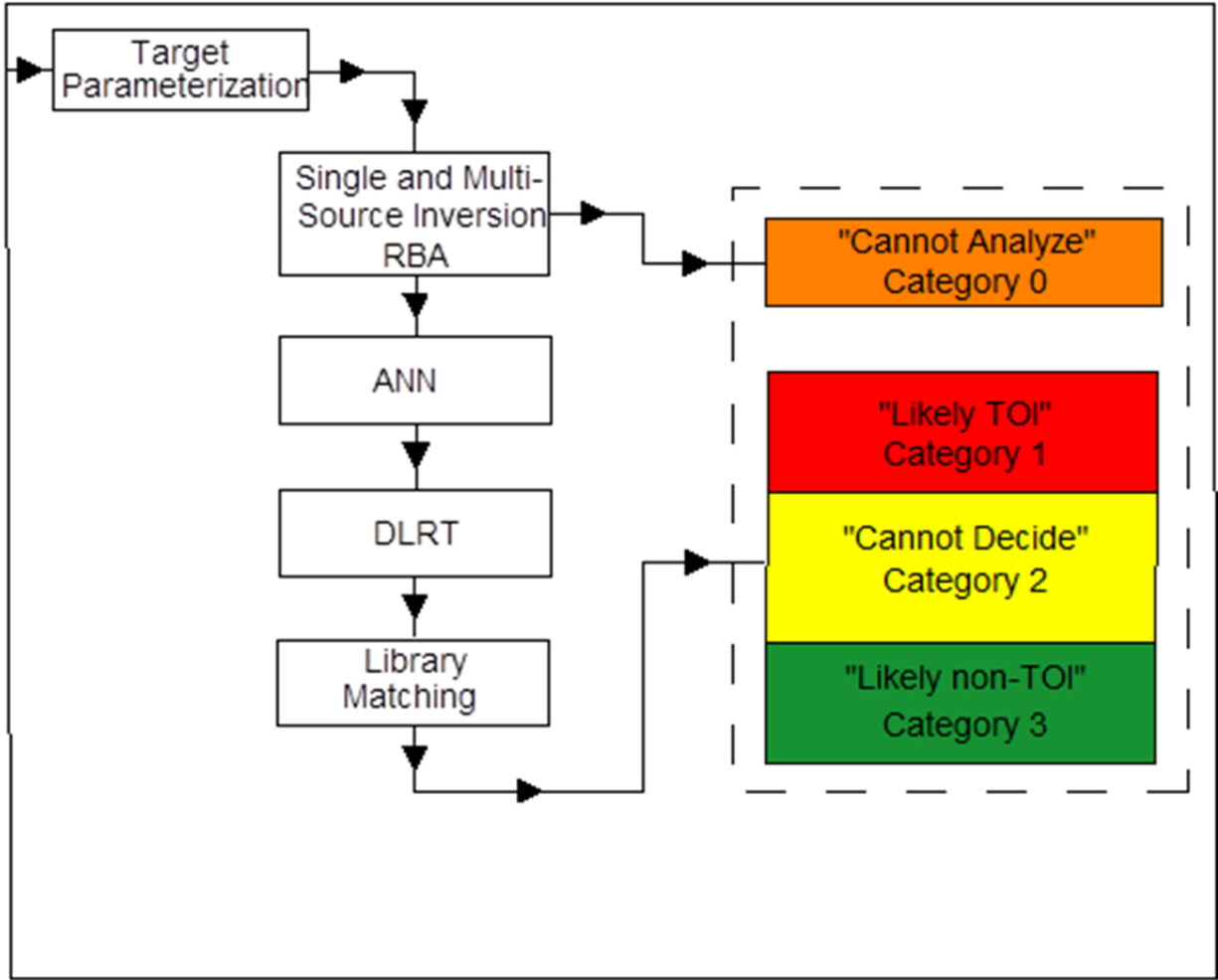
Figure 7. Simplified Block Diagram Illustrating the Processing Steps Used to Generate a Prioritized Dig List
