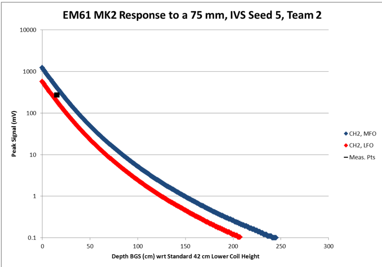
Figure 3. IVS LFO/MFO Plot for Team 2 for the 75mm Projectile Seed Item
