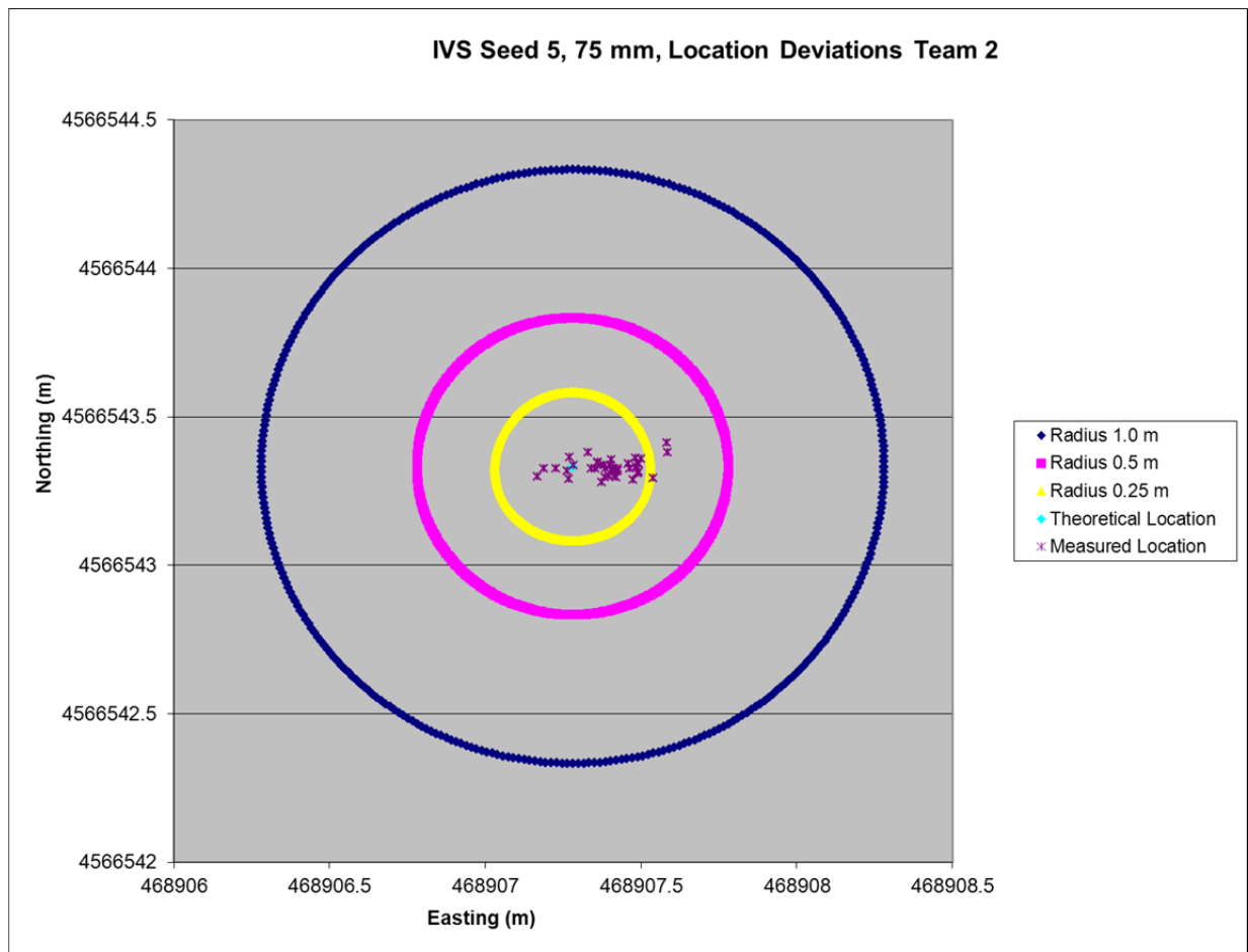
Figure 4. IVS Positioning Plot for Team 2 for the 75mm Projectile Seed Item
