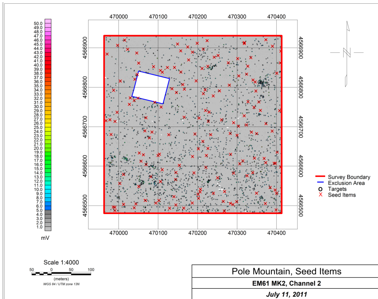
Figure 24. PMTMA EM61-MK2 Production Data With All 160 QC Seed Items Identified
