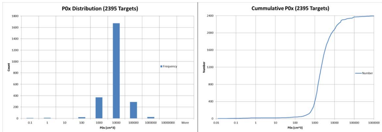
Figure 11. PMTMA Cued Production Data P_{0x} Statistics (Target Size)
