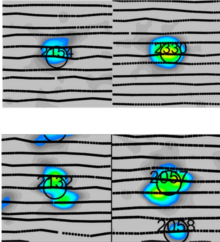
Figure 25. Footprints of targets 2154 and 2330 (37mm) and targets 2132 and 2057 (ISOs)
