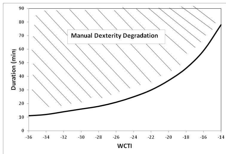
Figure 2-2. The left upper area (hatched) in the figure indicates combinations of WCTI and exposure durations for which the finger skin temperature will drop below 15°C (60°F) and manual dexterity will be impaired. For these experiments gloved hands were bared briefly before and during performing the dexterity tasks in the cold.
