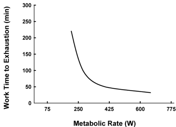
Figure 1-2. Influence of time-weighted metabolic rate (W) on work-time when wearing CBRNE protective clothing (closed) in hot weather in Soldiers with UCHS.
