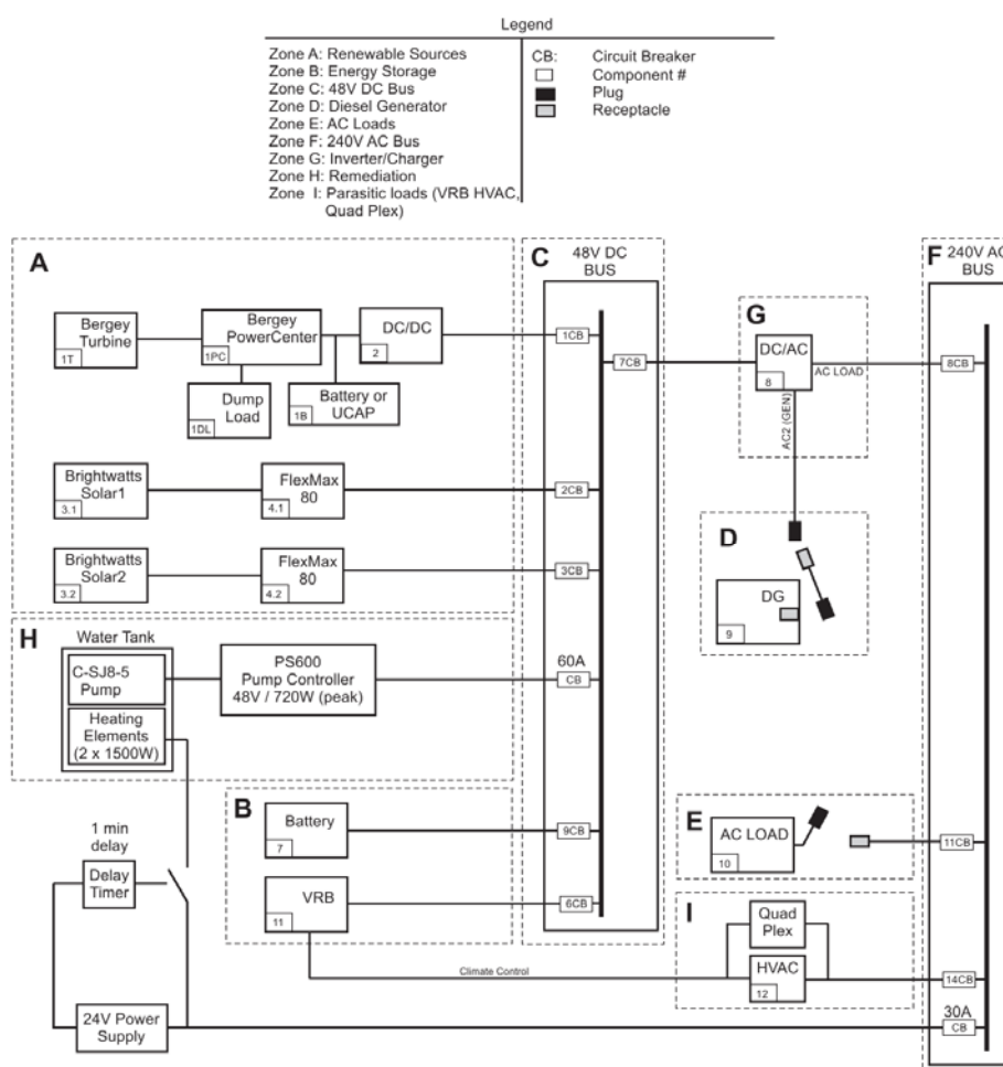
Fig. 1. Electrical schematic for microgrid system
