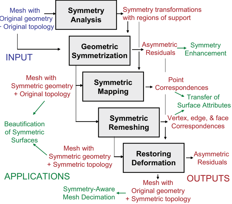
Figure 2.1: Symmetry-aware mesh processing framework.
