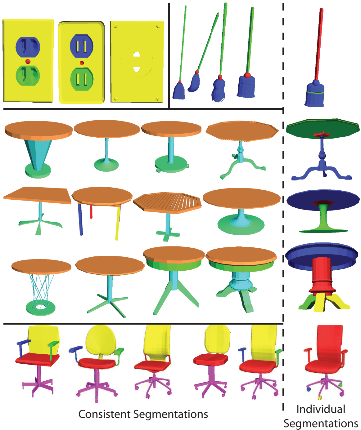
Figure 3.5: Results of consistent segmentations of several classes are shown to the left of the dotted line. Note that in many cases, the ability of our method to find outlier segments is helpful. To the right of the dotted lines are individual segmentations of the last models in the row. These individual segmentations fail to identify important segments that can be identified by comparing to other models in the class.
