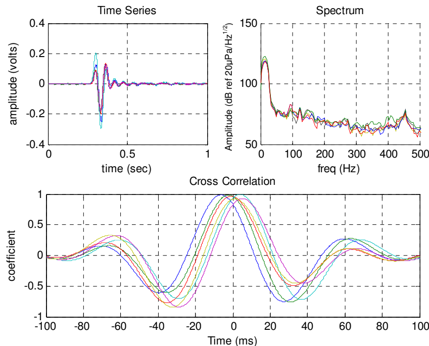
Figure 23: Example blast noise. This particular blast had a peak level of 120dB ref 20μPa. The cross-correlation (bottom) illustrates the measured phase delay between sensors. Note that all correlation peaks are about equal to 1 and fall within 5ms – the maximum possible acoustic propagation delay.
