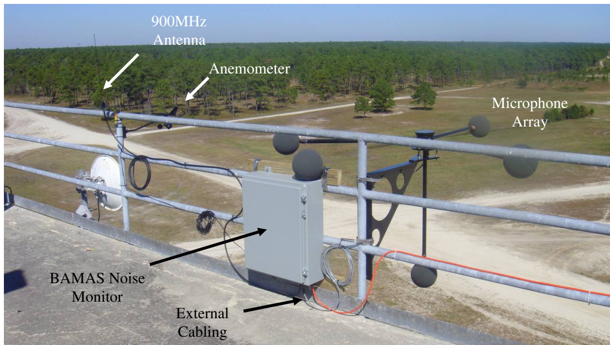
Figure 17: Node #2 Installation
