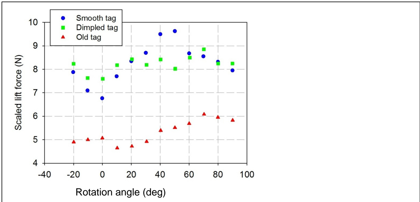
Fig. 10. Water tunnel results comparing scaled lift force versus rotation angle for the smooth, dimpled, and old tag at a constant flow speed of 5 m/s. The lift force is lower for the old tag over the entire range of flow orientations.
