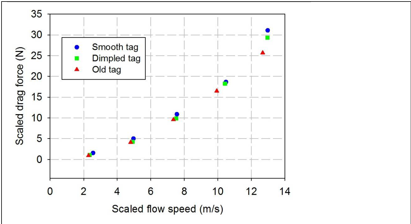
Fig. 7. Water tunnel test of the three tag models, showing scaled drag force versus scaled flow speed for the tag with its long axis parallel to the direction of flow ( 0^\circ rotation). Note that there is little difference between tag types in the scaled drag force over this range of flow speeds.
