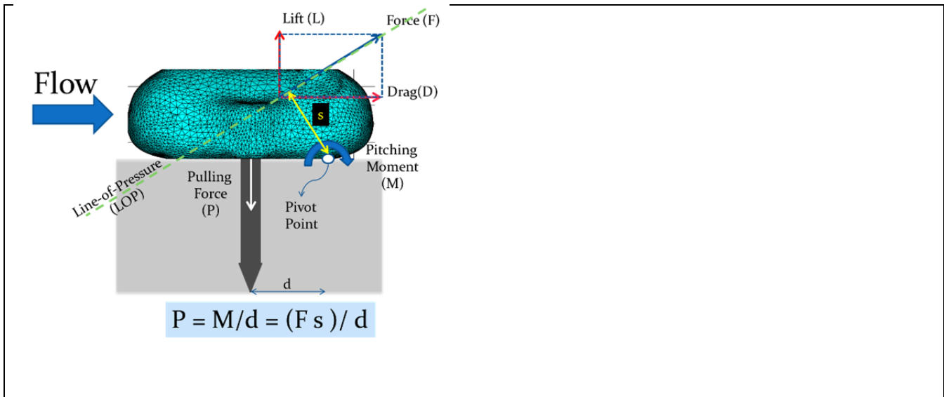
Fig. 1. Schematic illustrating the various forces and moments acting on the tag. Note that the pulling force 'P' is proportional to the pitching moment 'M'.
