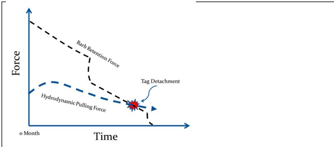
Fig. 4. Timeline of tag attachment failure based on CFD computations. Tag detaches when the pulling force equals the retention force of the darts.
