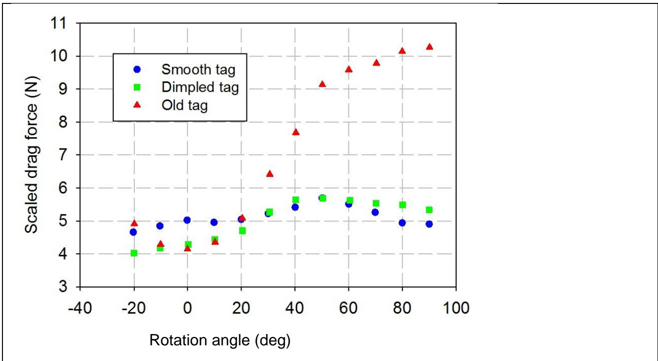
Fig. 8. Water tunnel results comparing the scaled drag force versus rotation for the three tags considered in this study at a flow speed of 5 m/s. Note that at flow orientations greater than \pm 30^\circ , the old tag produces considerably greater drag.
