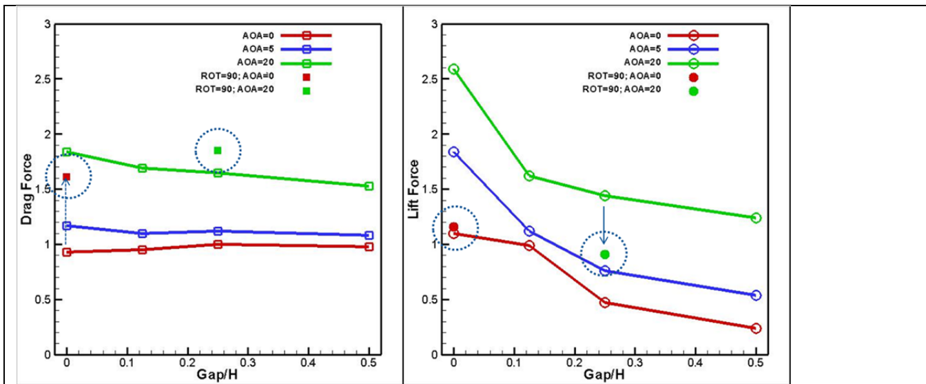
Fig. 2. The effect of varying gap, angle of attack (AOA) and orientation (rotation) on the drag and lift forces on the tag.
