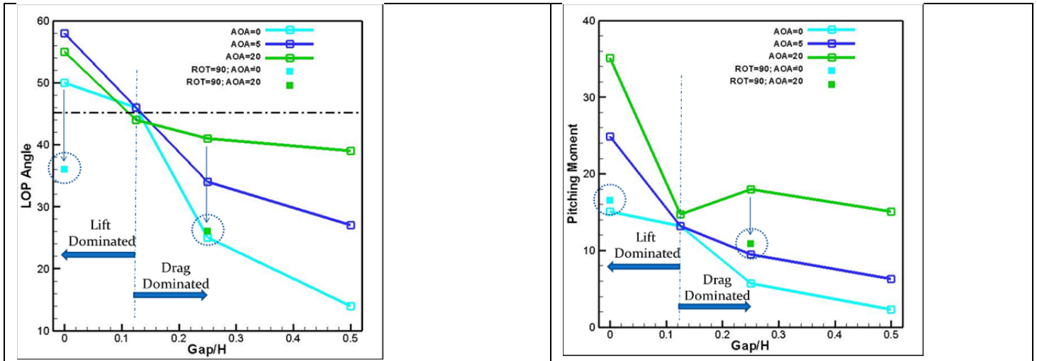
Fig. 3. Effect of gap, AOA and orientation on the direction of the net force (left panel) and pitching up moment (right panel) on the tag.
