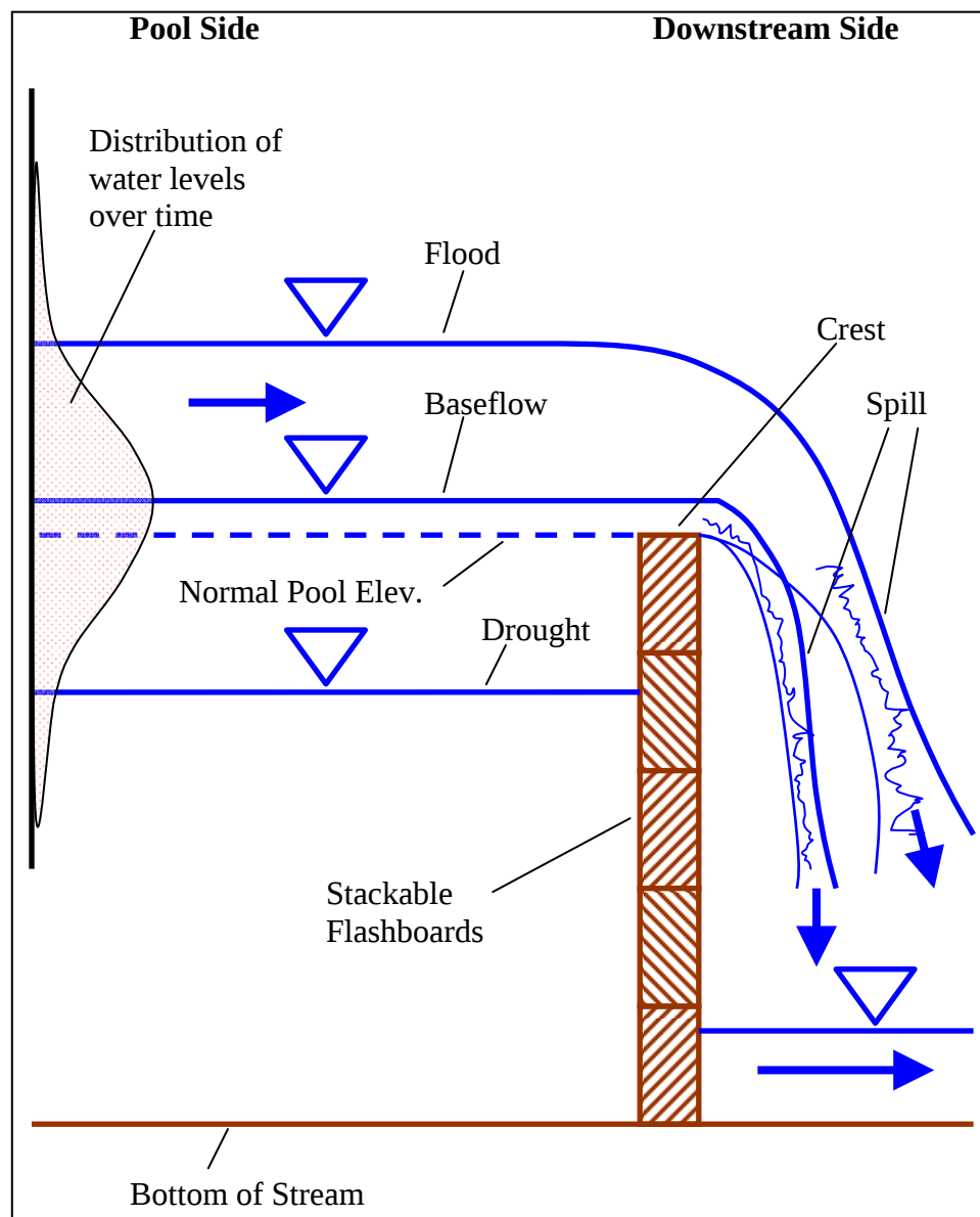
Figure D12. Flashboard Weir.
