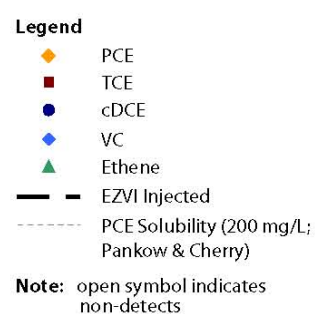
VOC Trends in Downgradient Wells (ML-7) Site 45, Parris Island MCRD, Parris Island, SC
