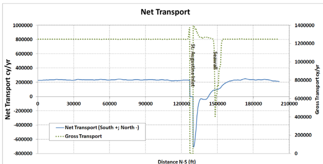
Figure 11. Final calibration of the calculated net sand transport rate for the calibration period of 1986-1999, including modified waves over the downdrift (south) side of the inlet from R123-R132.
