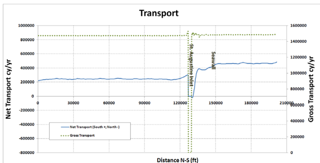
Figure 10. Initial calibration of the calculated net sand transport rate for the calibration period of 1986-1999.
