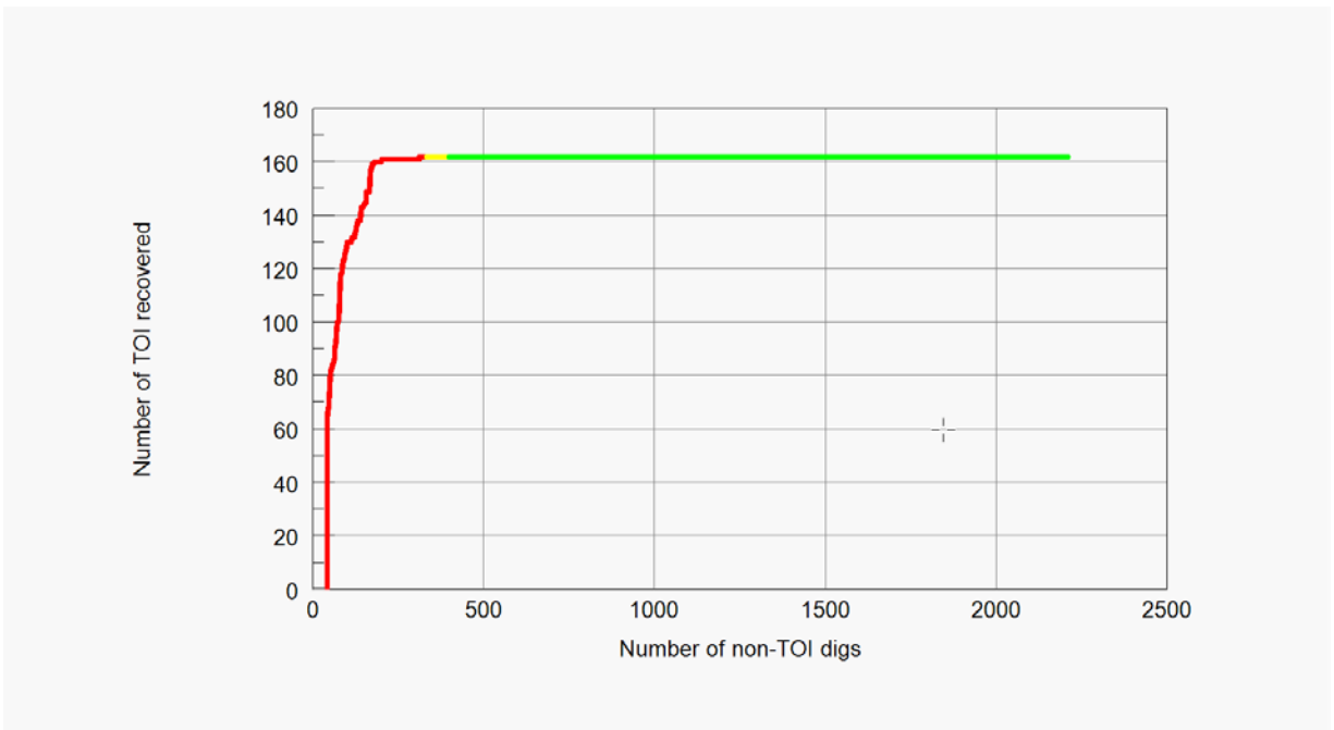
Figure 13: ROC curve for most aggressive readjustment of bsum parameter
