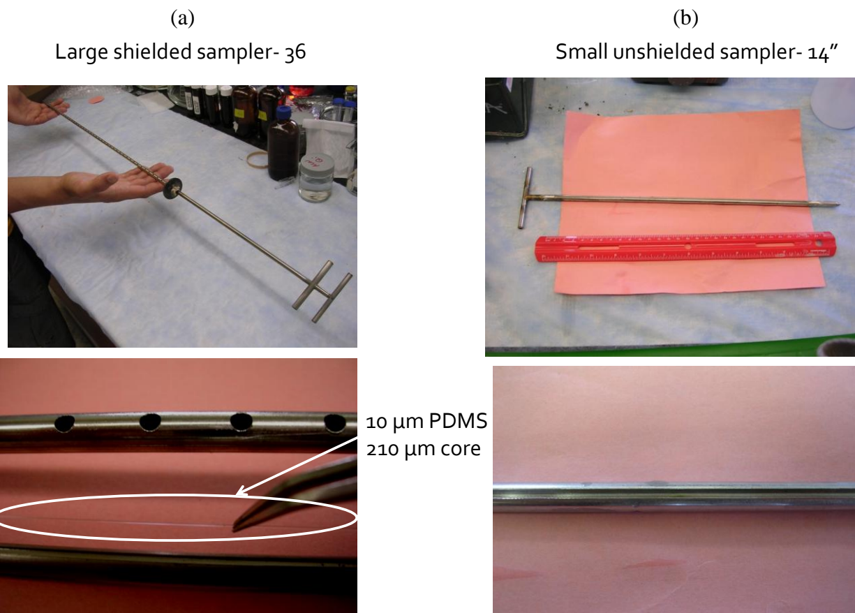
Figure 1. Shielded and unshielded holders for SPME fiber.
