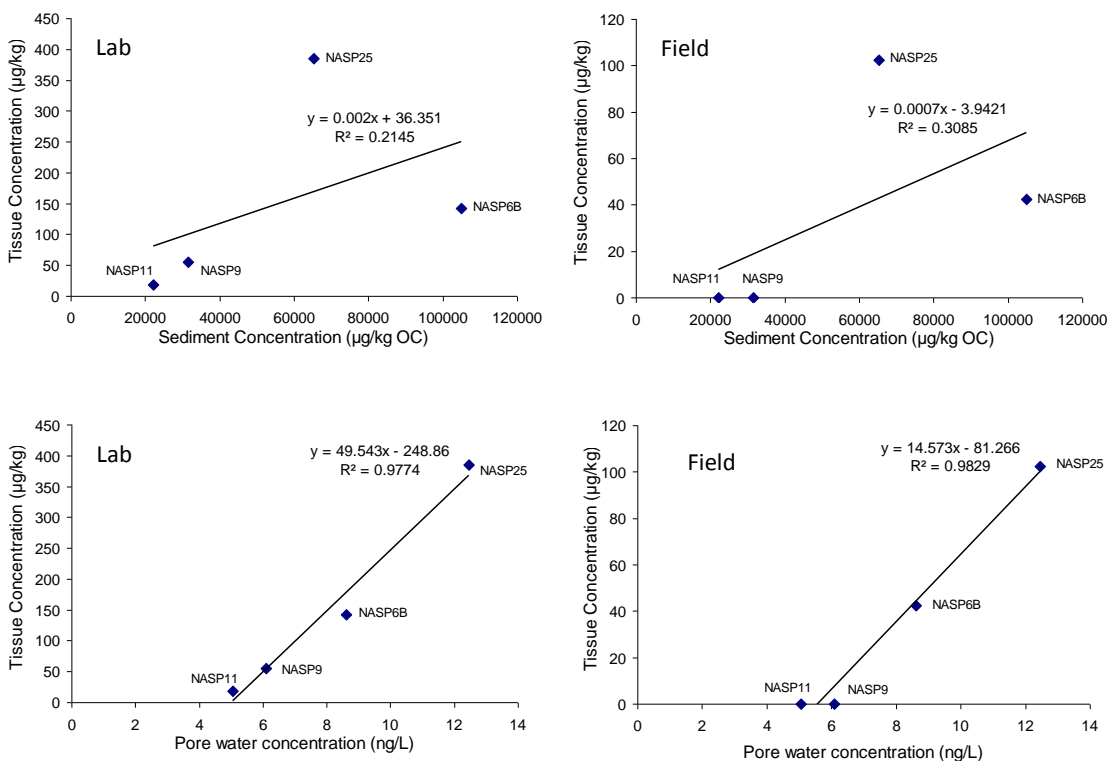
Figure 13. Uptake of PAHs from 96 h exposures with the amphipod Leptocheirus plumulosus in both lab (left) and in situ (right).
