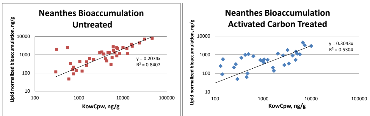
Figure 10. Bioaccumulation as a function of PDMS-measured porewater concentration for both untreated (left) and activated carbon treated (right) microcosms (all measured PCB congeners)
