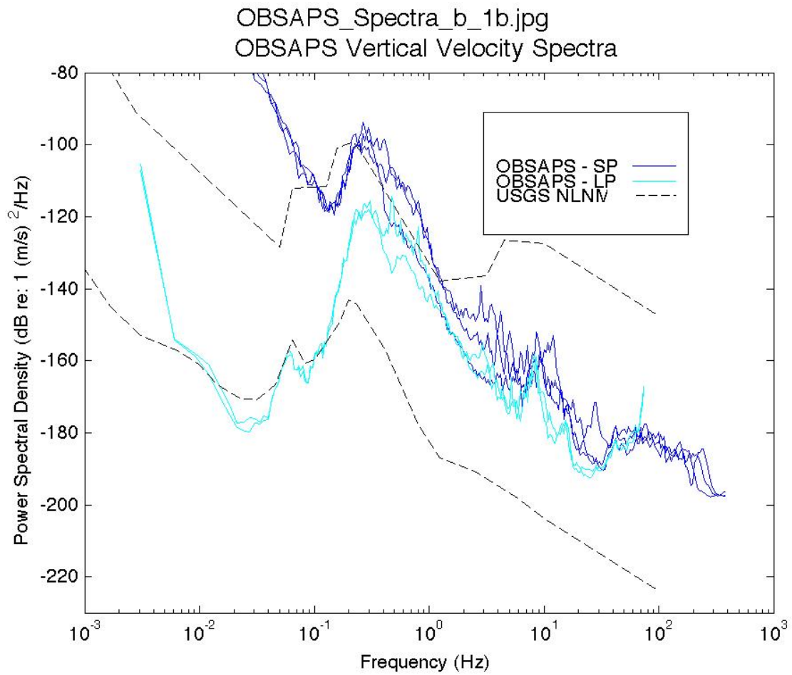
Figure 3: Samples of vertical particle velocity spectra for the three short-period and two long-period OBSs on OBSAPS. The discrepancy at the microseism peak needs to be fixed. Figure from Stephen et al (in press).
