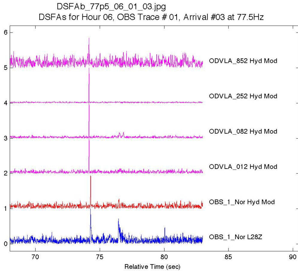
Figure 2 - DSFA Example #1: Here we compare receptions for a single 77.5Hz M-sequence on six OBSAPS receivers: (from bottom to top) the vertical geophone on the North OBS (blue), the hydrophone module on the North OBS (red), and the hydrophone modules on the O-DVLA at 12, 82, 252 and 852m above the seafloor (magenta). The range to the North OBS (bottom two traces) was 31.4km and the range to the O-DVLA (top four traces) was 30.3km. We call the large peak near 74sec the "PE predicted" arrival because it is consistently a large arrival across all of the receivers. The strong arrival about 3sec later on the vertical geophone on the OBS is a classic DSFA, although it is strange that this arrival is so weak on the co-located hydrophone module. There is a weak indication of this arrival on the O-DVLA up to at least 82m above the seafloor. There is also a weak indication of second DSFA on the geophone channel near 80sec. Figure from Stephen et al (in press).
