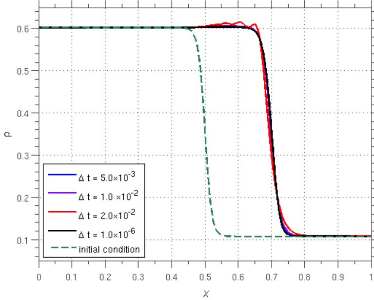
Figure 14: Solution of the propagating wave problem at t = 0.2 for time step sizes of \Delta t = 5.0 \times 10^{-3} , \Delta t = 1.0 \times 10^{-2} , \Delta t = 2.0 \times 10^{-2} , and \Delta t = 1.0 \times 10^{-6} (reference solution) when \Delta x = 1.0 \times 10^{-2} , \text{Re} = 2.0 \times 10^2 , and \text{We} = 1.0 \times 10^4 .
