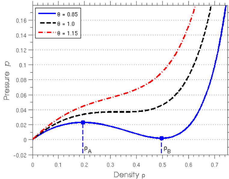
Figure 1: Pressure as a function of density at temperatures \theta = 0.85, 1.0, and 1.15 . At \theta = 0.85 , the elliptic region, defined as the range where the pressure function is monotonically decreasing with respect to the density field, is (\rho_A, \rho_B) = (0.194, 0.496) .
