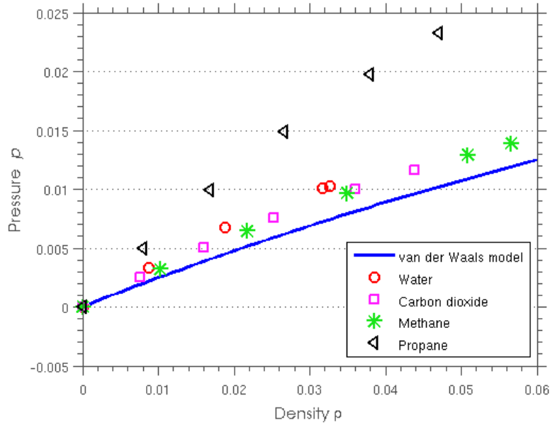
Figure 3: Detailed comparison of van der Waals fluid model with real materials at \theta = 0.85 in vapor phase. The data for water, carbon dioxide, methane, and propane are obtained from [1] and scaled to dimensionless form.
