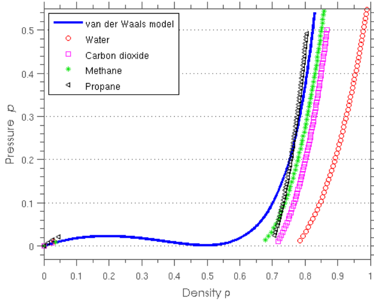
Figure 2: Comparison of van der Waals fluid model with real materials at \theta = 0.85 . The data for water, carbon dioxide, methane, and propane are obtained from [1] and scaled to dimensionless form.
