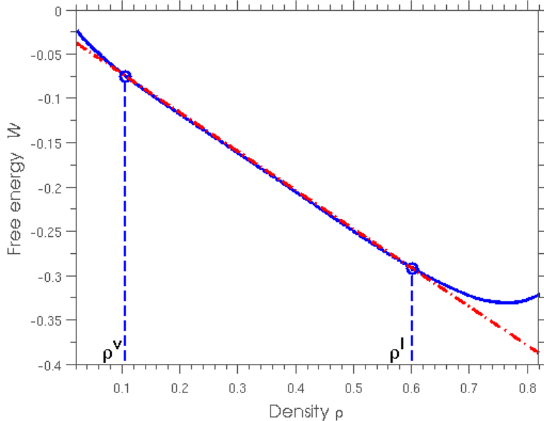
Figure 4: The isothermal free energy W as a function of density \rho at \theta = 0.85 is plotted as the blue solid line. The red dash-dotted line is the common tangent line passing through the Maxwell states (\rho^v, W(\rho^v)) and (\rho^l, W(\rho^l)) , which are marked as blue circles.
