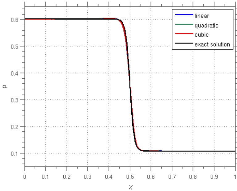
Figure 12: Solution of the stationary wave problem at t = 0.1 using linear, quadratic, and cubic NURBS for \Delta x = 1.0 \times 10^{-2} , \Delta t = 1.0 \times 10^{-6} , \mathbb{R}e = 2.0 \times 10^2 , and \mathbb{W}e = 1.0 \times 10^4 .
