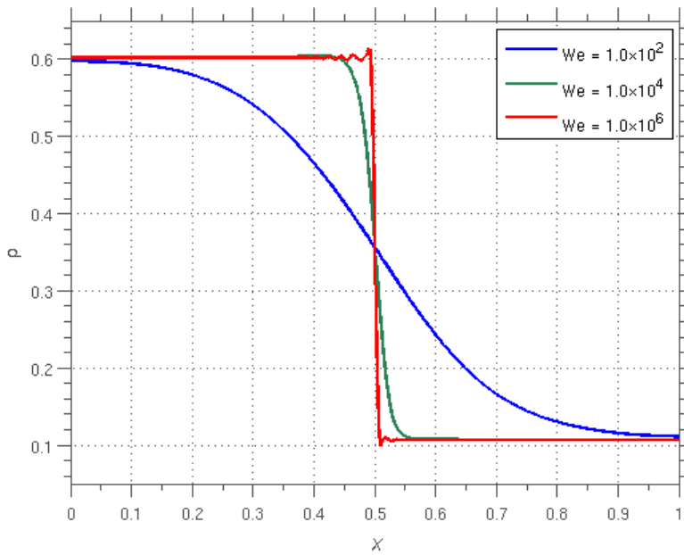
Figure 13: Solution of the stationary wave problem at t = 0.1 for Weber numbers 1.0 \times 10^2 , 1.0 \times 10^4 , and 1.0 \times 10^6 when \Delta x = 1.0 \times 10^{-2} , \Delta t = 1.0 \times 10^{-6} , and \mathbb{R}e = 2.0 \times 10^2 .
