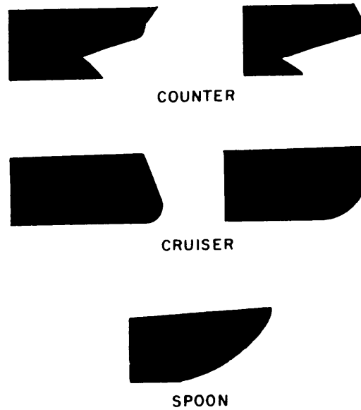
Figure 30.—Stern designs.
