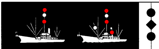
VESSEL RESTRICTED IN ABILITY TO MANEUVER (SPECIAL OPERATIONS), EXCEPT VESSEL ENGAGED IN MINESWEEPING- LEFT, NOT MAKING WAY; RIGHT, MAKING WAY
