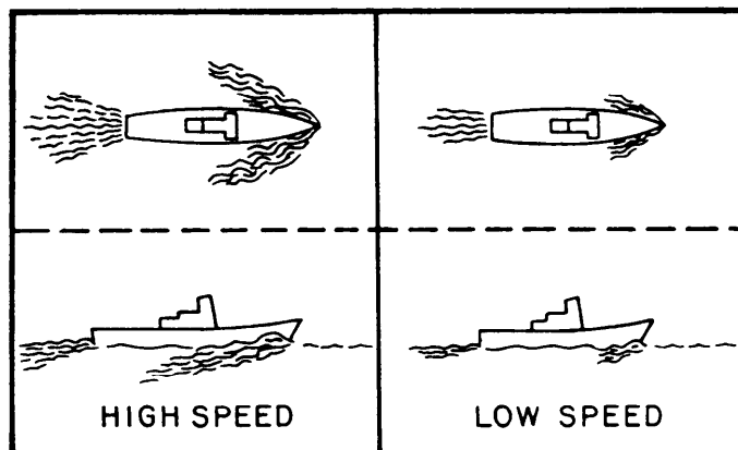
Figure 13.—Bow wave and stern wake.
