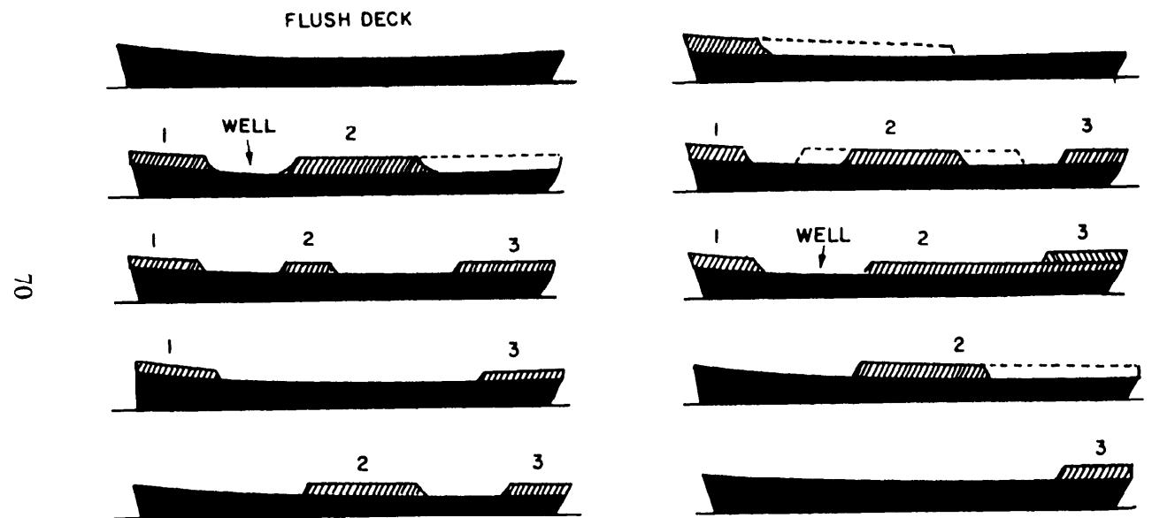
Figure 28.—Basic hull designs.
