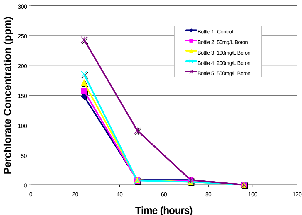
Figure 15. Boron Bottle Test Results
