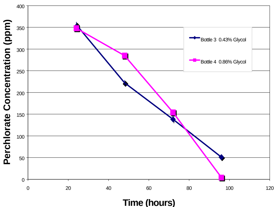
Figure 8. Glycol Bottle Test Results without CBP Nutrient
