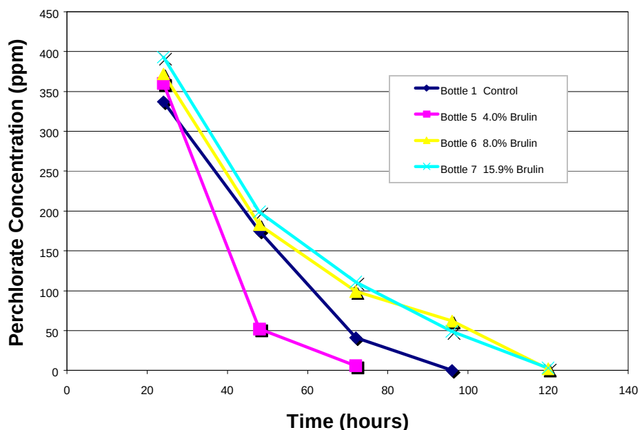
Figure 12. Brulin Bottle Test Results using 0.8 g/l CBP
