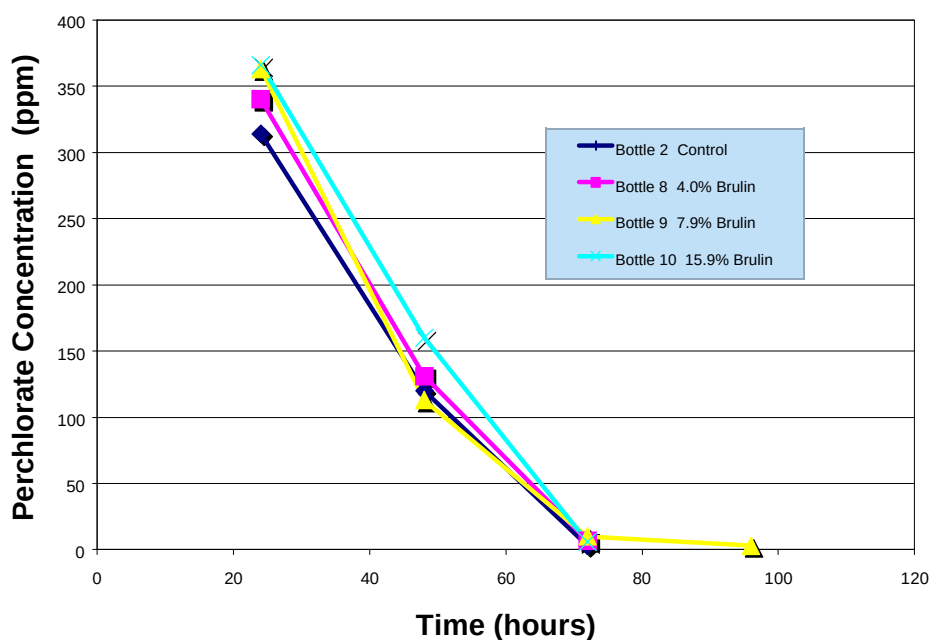
Figure 13. Brulin Bottle Test Results with 1.6 g/l CBP
