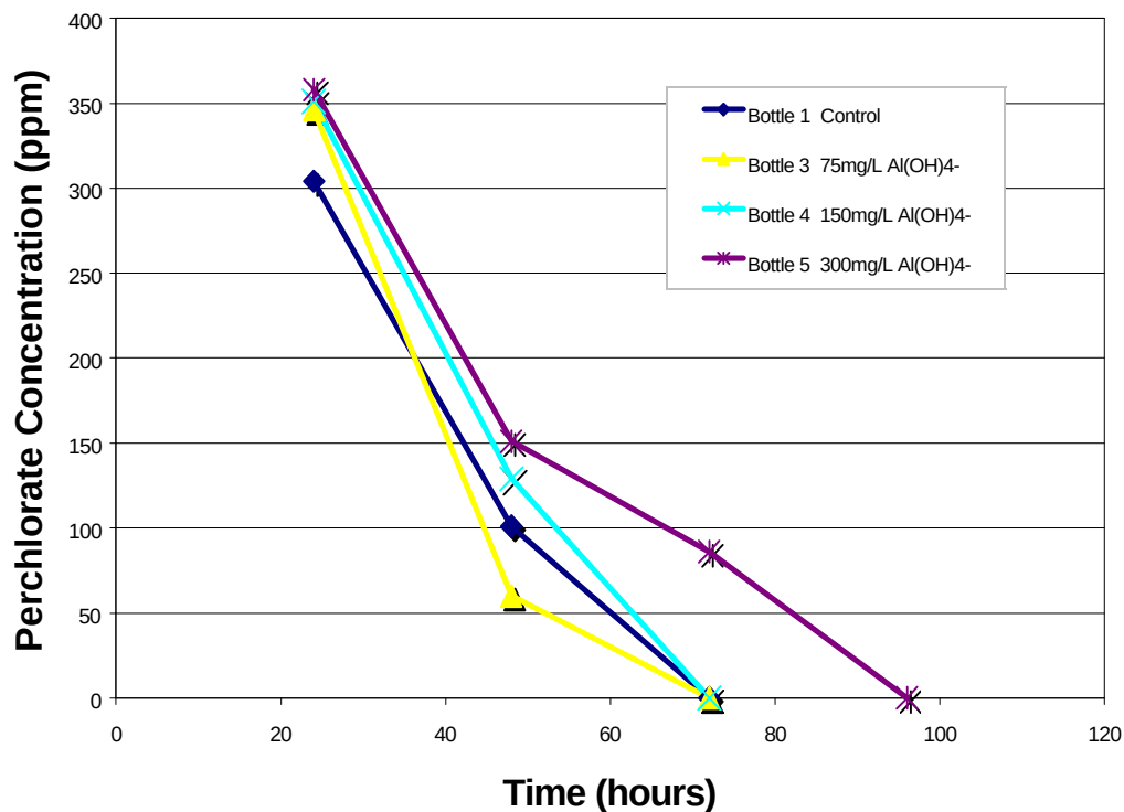
Figure 17. Aluminum Hydroxide Test Results with 0.9 g/l CBP Nutrient
