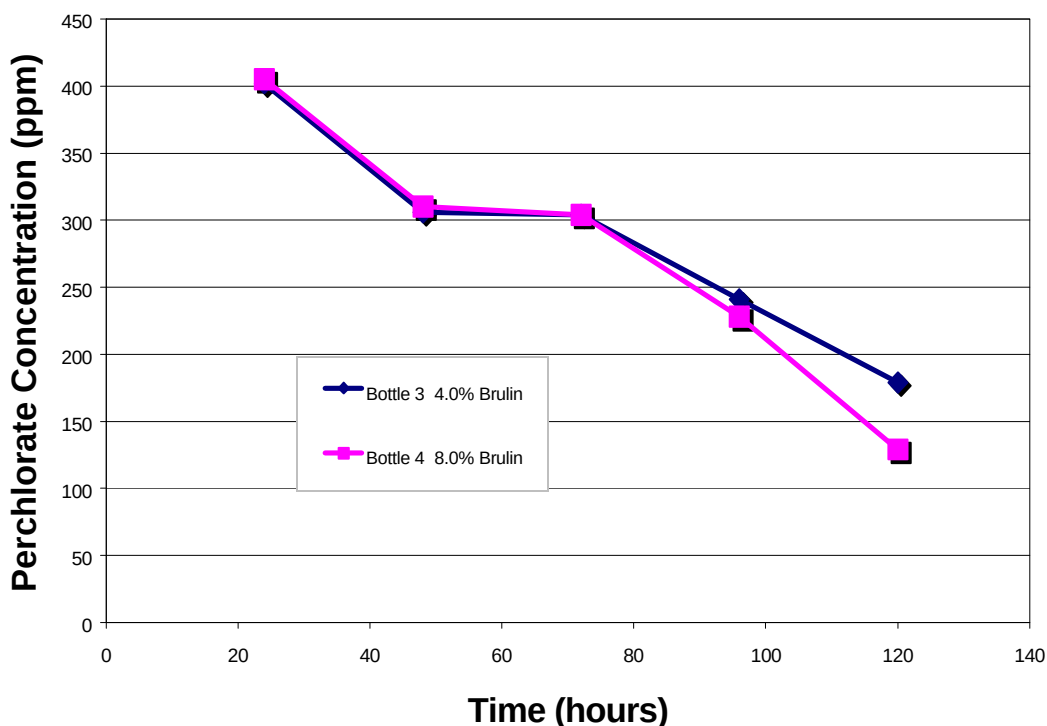
Figure 14. Brulin Bottle Test Results without CBP Nutrient
