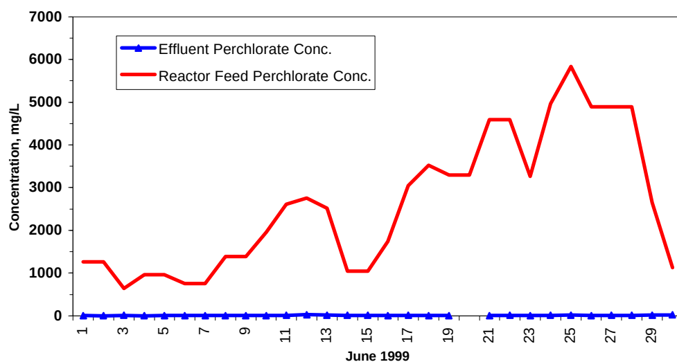
Figure 20. Variation of Perchlorate Concentration in Reactor Feed Composite
