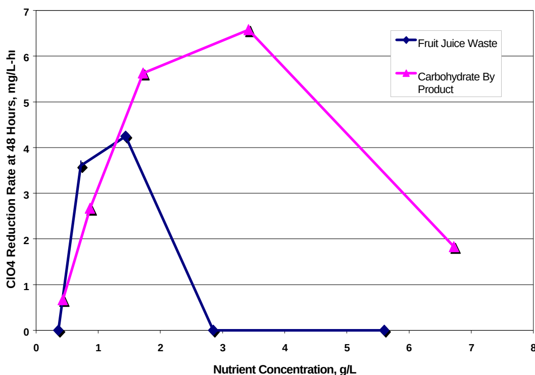
Figure 5. Comparison of Nutrient Performance
