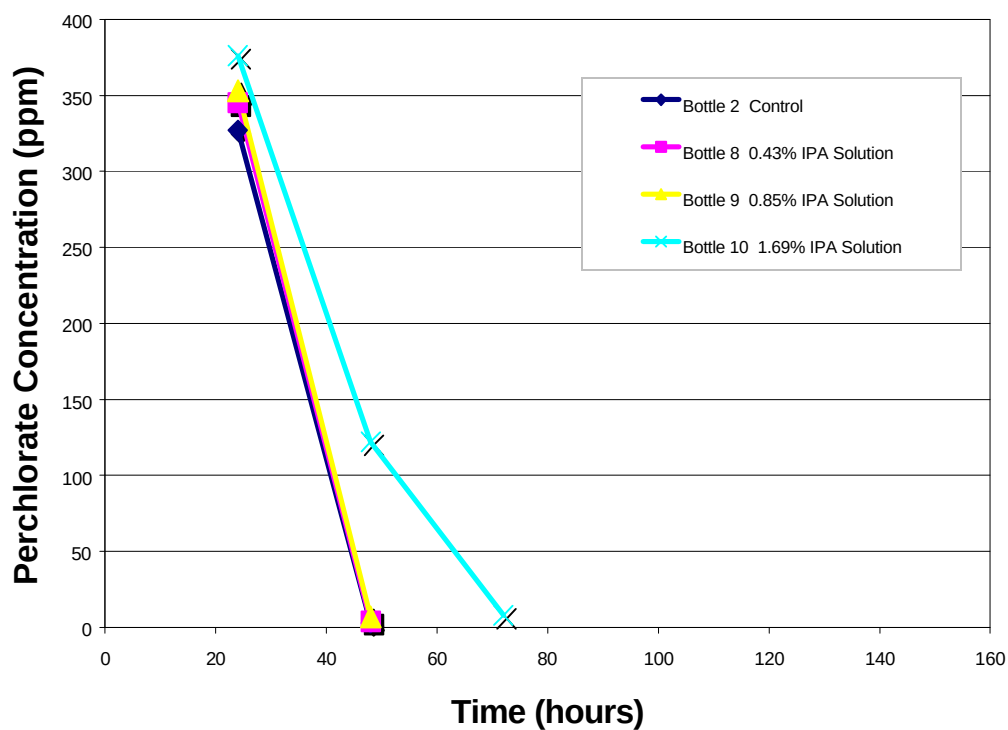
Figure 10. Isopropyl Alcohol Bottle Test Results with 1.7 g/l CBP Nutrient
