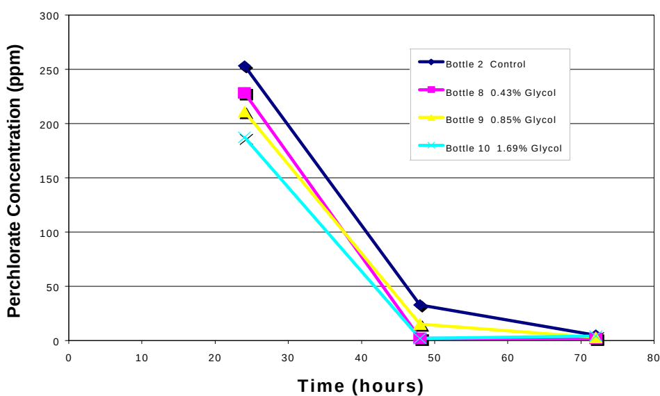
Figure 7. Glycol Bottle Test Results with 1.7 g/l CBP Nutrient
