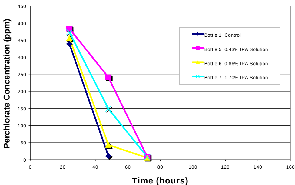
Figure 9. Isopropyl Alcohol Bottle Test Results with 0.9 g/l CBP Nutrient
