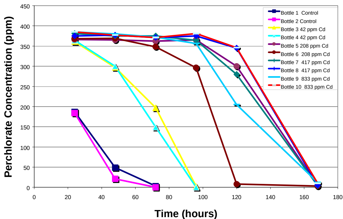
Figure 16. Cadmium Bottle Test Results
