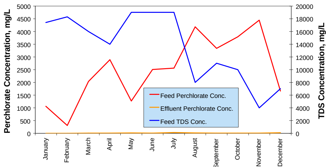
Figure 19. Reactor Perchlorate and TDS Concentration
