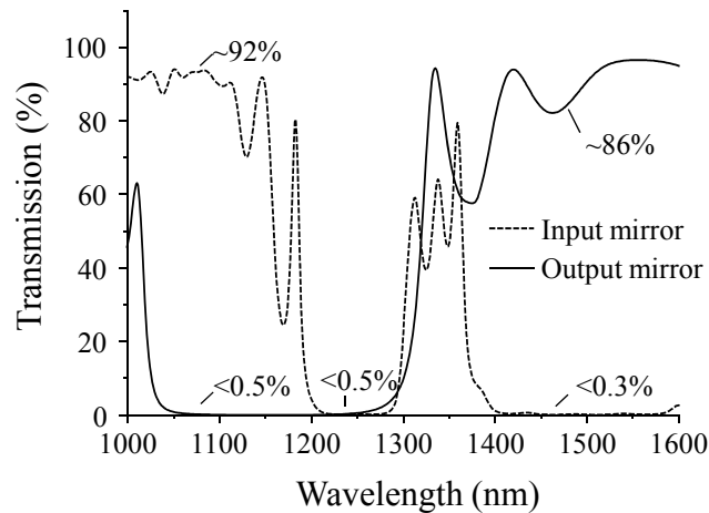
Figure 3. Transmission spectra for the input and output mirrors of the eye-safe diamond Raman lasers.
