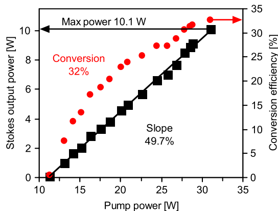
Fig. 2. (Color online) Slope and conversion efficiency of the diamond Raman laser as a function of incident pump power.
