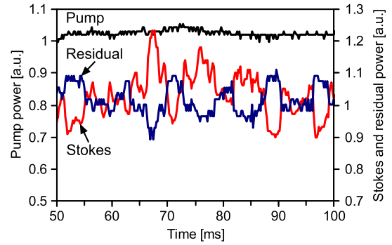
Fig. 3. (Color online) Temporal characteristics of pump, residual pump, and Stokes output radiation.
