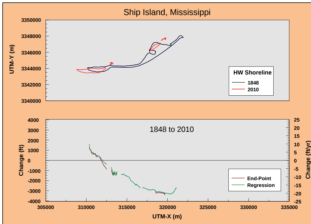
Figure C34. Change in historical shoreline position, Ship Island, MS, 1848 to 2010.
