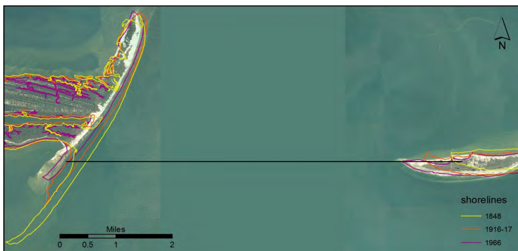
Figure 4.13. Transect location for illustrating historical inlet cross-sections for Ship Island Pass.
