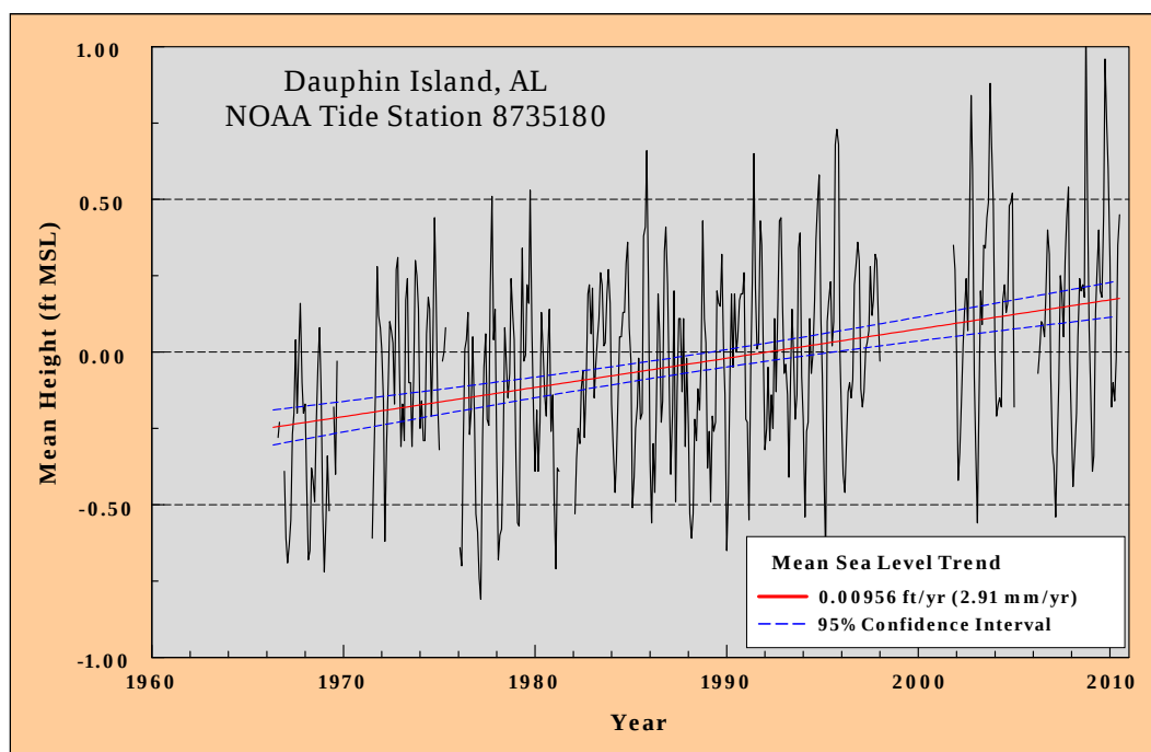
Figure 3.16. Monthly mean water level measurements and sea-level rise trend at Dauphin Island, AL gauge 8735180, 1966 to 2010.
