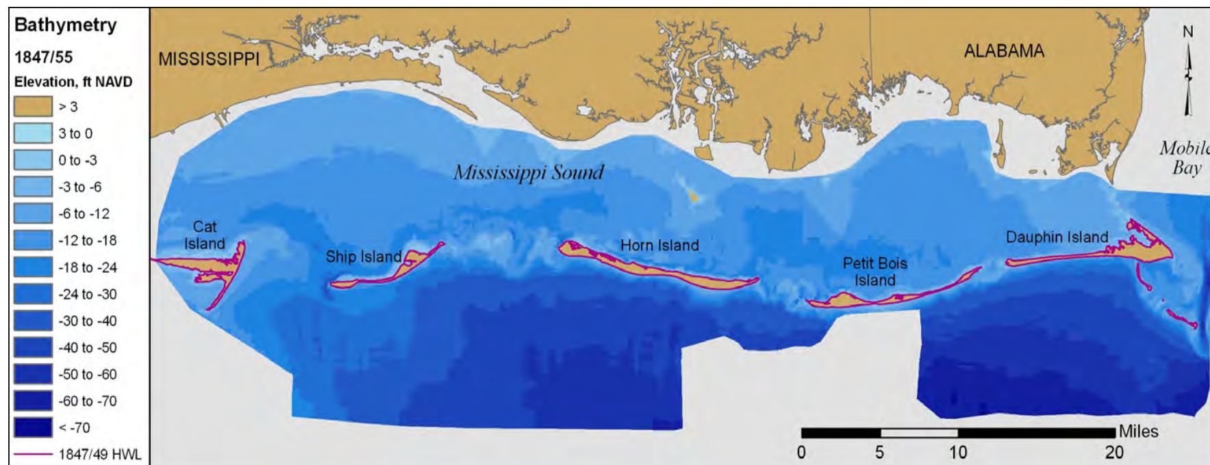
Figure 4.1. Regional bathymetric surface for the study area, 1847/55.
