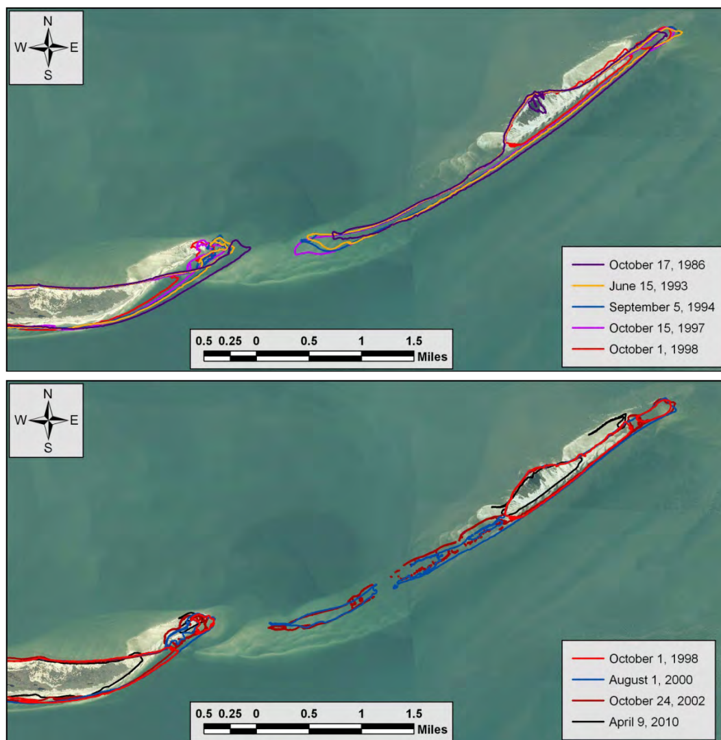
Figure 3.7. High-water shoreline position for Ship Island, MS (1986 to 2010), illustrating sand spit growth and dispersion along the western end of East Ship Island. Background imagery was flown October 1, 2008.
