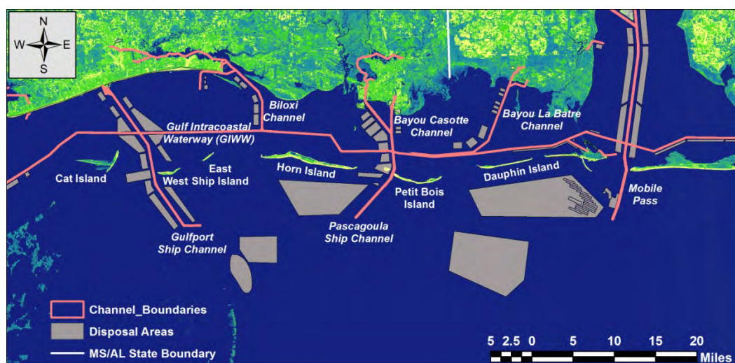
Figure 1.3. Mississippi and Alabama coastal deposits illustrating the barrier island system west of Mobile Pass, including navigation channels and dredged material disposal areas. Background image was acquired via Landsat on February 2, 2010.
