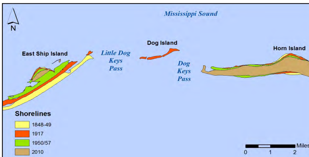
Figure 3.11. Composite island changes for western Horn Island and East Ship Island, 1848 to 2010.
