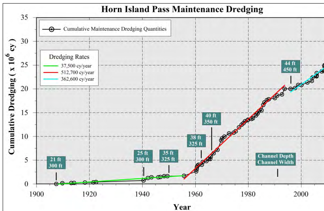
Figure 2.3. Cumulative maintenance dredging volumes and associated sand dredging rates for Horn Island Pass.
