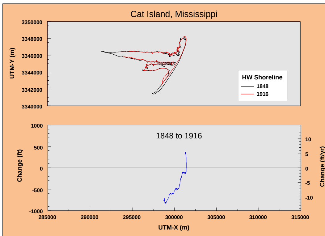
Figure C35. Change in historical shoreline position, Cat Island, MS, 1848 to 1916.
