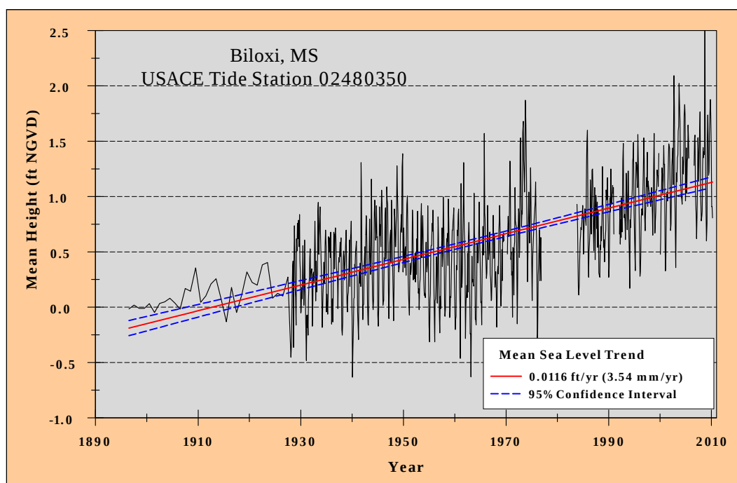
Figure 3.15. Mean annual and monthly water level measurements and sea-level rise trend at Biloxi, MS gauge 02480350, 1896 to 2010.
