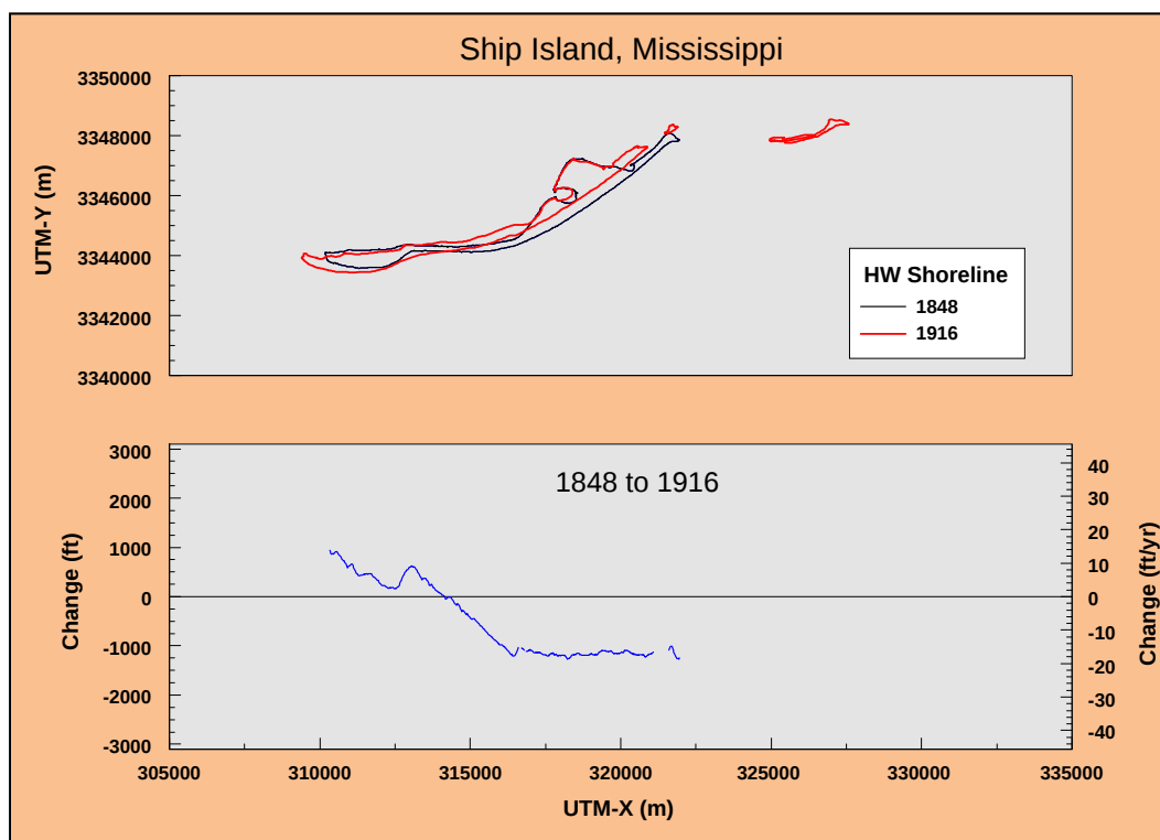
Figure C26. Change in historical shoreline position, Ship Island, MS, 1848 to 1916.
