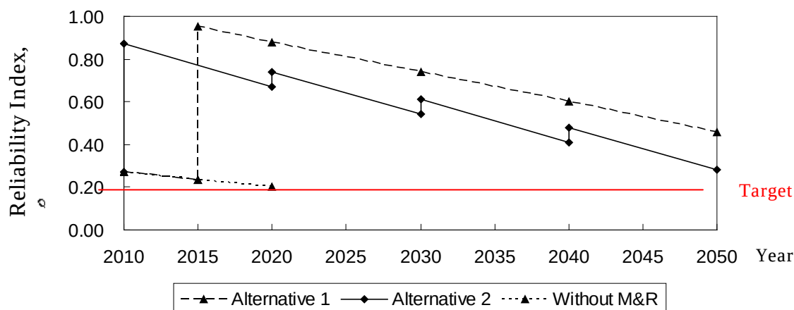
Figure 7. Time-dependent reliability index profiles.
