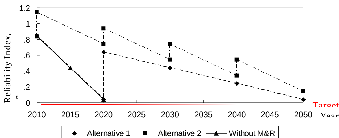
Figure 9. Time-dependent reliability index profiles.
