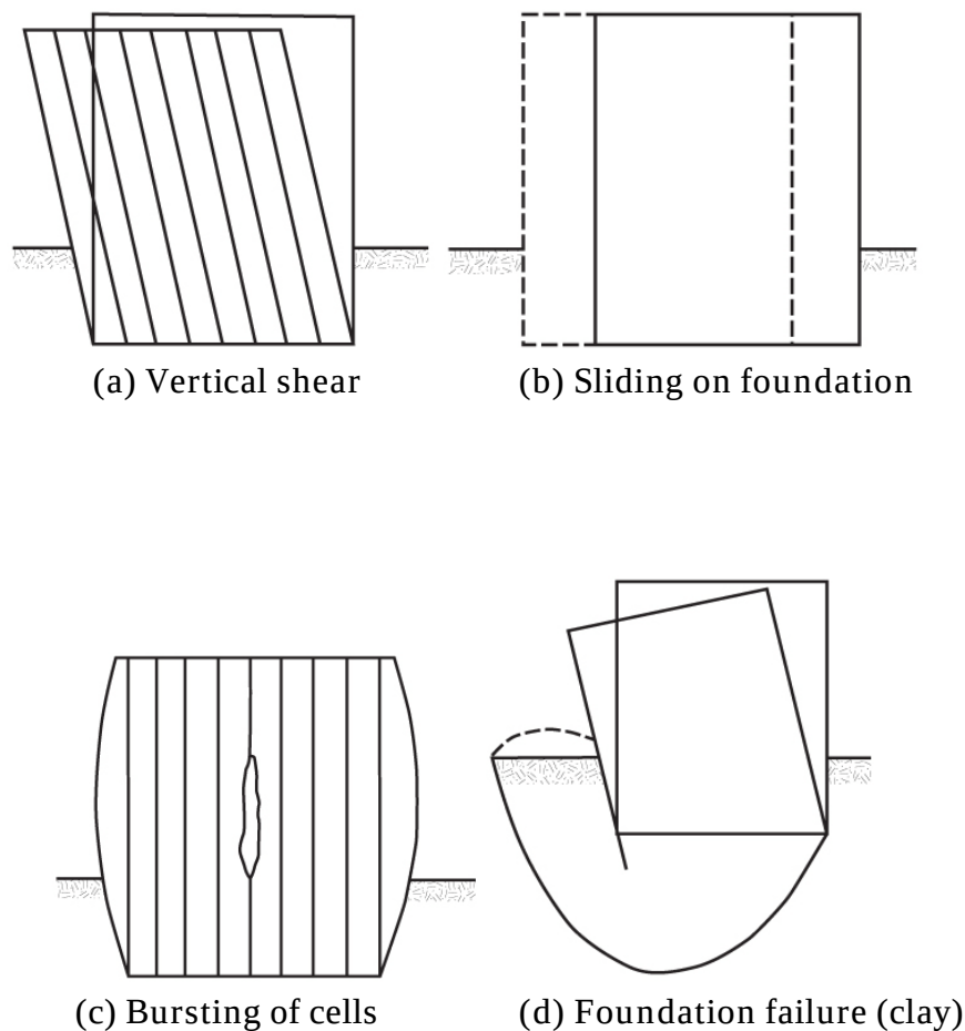
Figure 4. Failure modes for cellular structures (adapted from Asker 1988).
