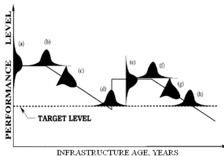
Figure 5. Reliability index profile of an infrastructure with M&R (adapted from Frangopol et al. 2001).
