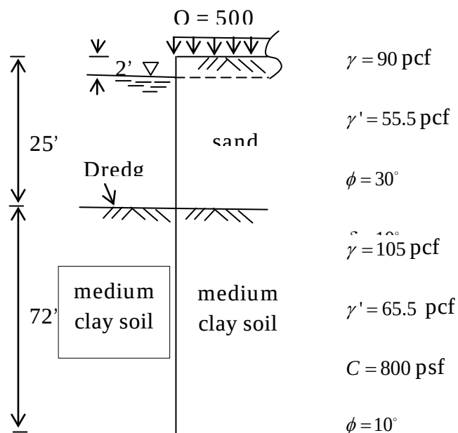
Figure 6. Cantilever wall in cohesive soil (adapted from Asker 1988).
