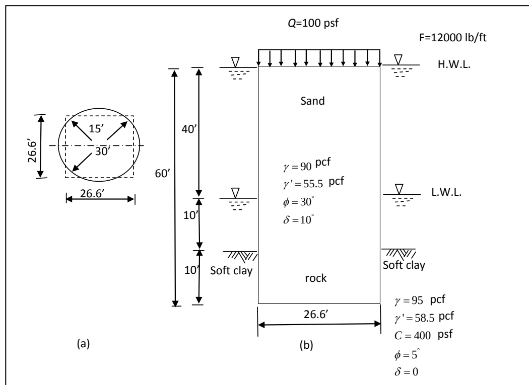
Figure 8. Single cell on rock foundation: (a) plan; (b) cross section.
