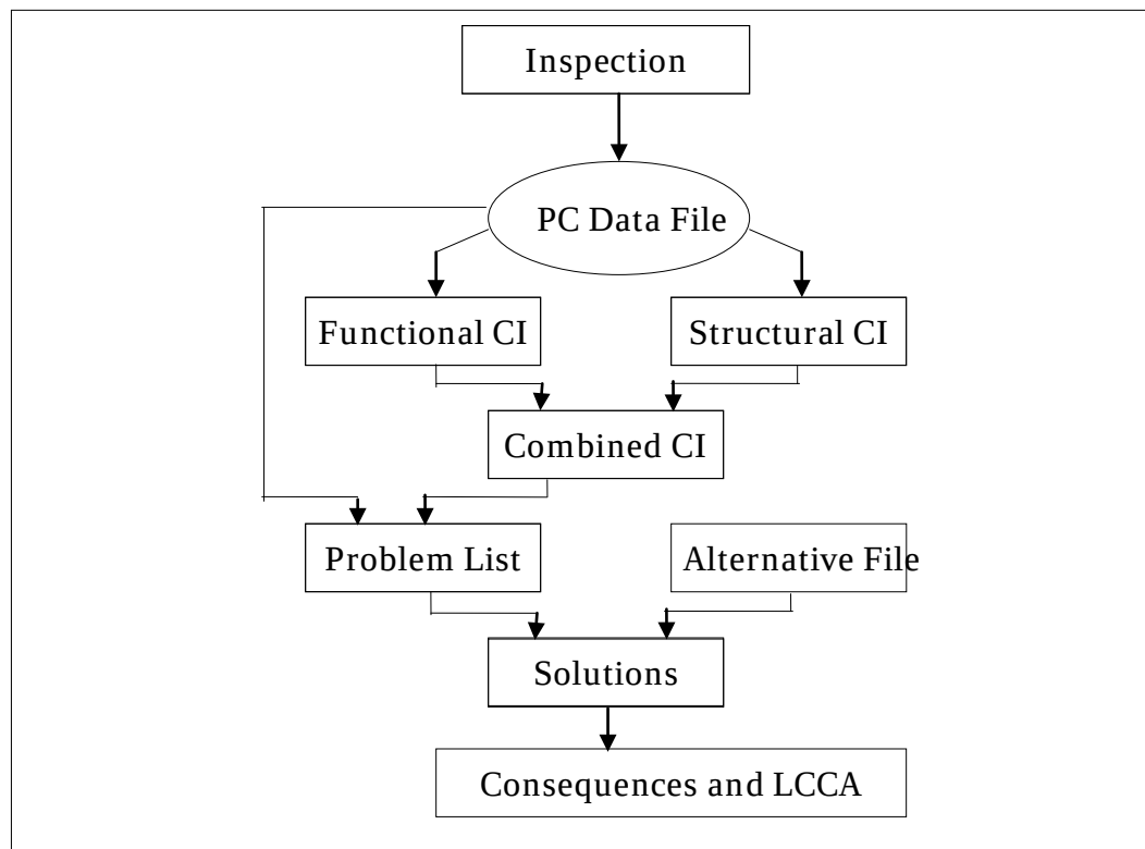
Figure 1. Schematic of historic inspection, maintenance, and repair analysis of steel sheet pile.
