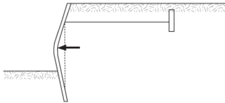
(a) Failure of piling in bending
