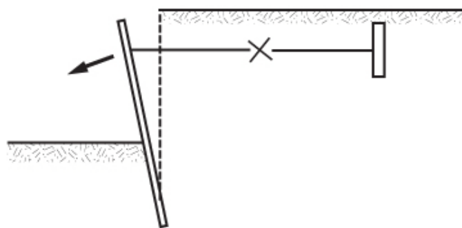
(c) Failure of anchor rod (anchored walls only)
