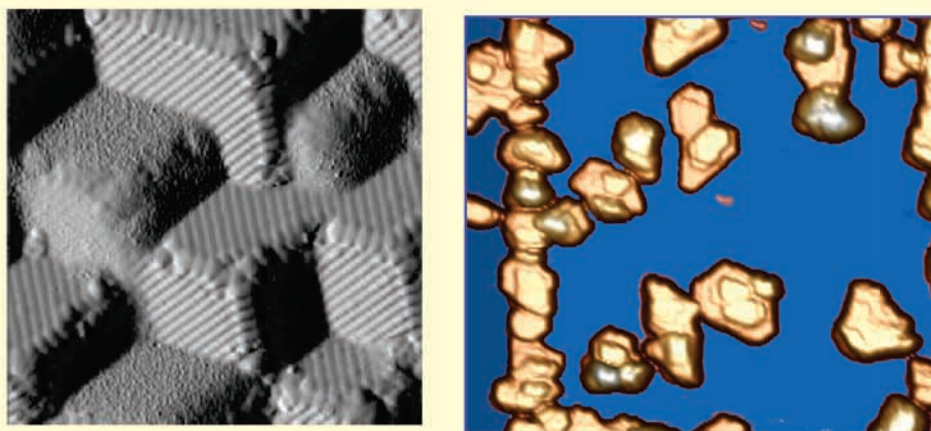
Left: STM image of faceted Pd/W(111) (15 nm x 15 nm)—Rows of individual atoms are visible on the flat faces of the three-dimensional nanoarchitecture of a faceted W surface. Right: STM image (200 nm x 200 nm)—Ruthenium nanoparticles on a graphite substrate (courtesy of T. Madey, Rutgers Univ., and J. Hrbek, Brookhaven National Laboratory).
