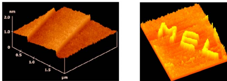
Figure 6.4. Measured step heights in Si (left) and line-width measurement and control in Si (right), after Ted Varburger and Richard Silver, NIST (courtesy of NIST) [5].
