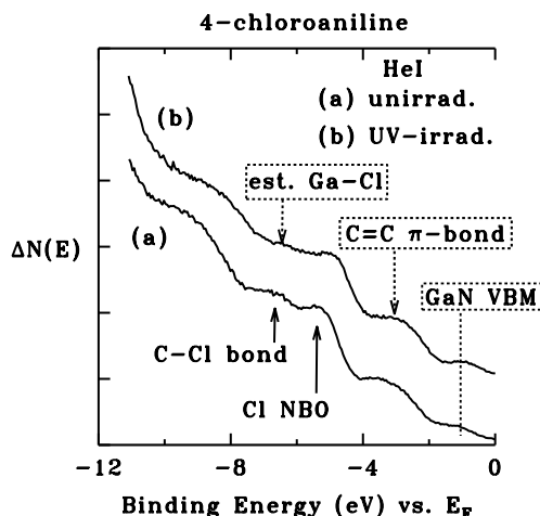
Fig. 7. Similar to Fig. 5b and c but using HeI excitation. Each data set was obtained in a single scan at 0.40 eV resolution. The position of the GaN VBM on the adsorbate-covered surface is indicated. The intensity above the GaN VBM is due to higher-energy satellites in the HeI spectrum and to HeII-excited photoemission features. The increasing intensity toward higher BE results from slow-secondary electron emission. Peaks are labelled which derive a large part of their intensity from C–Cl \sigma -bonding and Cl NBOs. Also shown is the estimated position of the Ga–Cl bonding orbital, based on data for \text{Cl}_2/\text{GaAs}(110) in Ref. [38]. See text for details.
