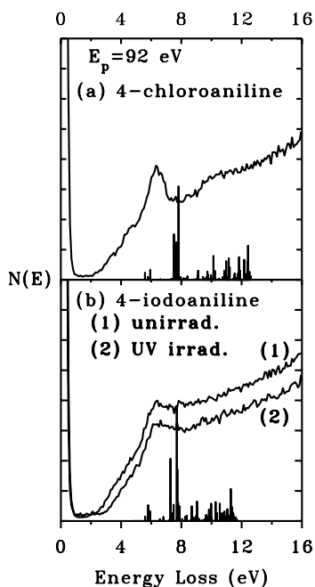
Fig. 3. Surface-sensitive ELS data (92 eV primary beam) for GaN(0001) after exposure to (a) 4-chloroaniline and (b) 4-iodoaniline. In (b), the effect of Hg-arc radiation is shown. Relative intensities are quantitative. The instrumental resolution (full-width at half-maximum of the elastic peak) is 0.5 eV. The vertical lines give the results of CIS calculations (up to ~12 eV) of the optical absorption spectra of the free molecules (see text).
