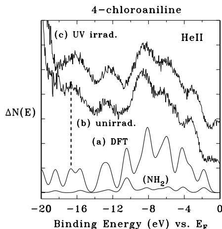
Fig. 5. HeII UPS ( h\nu = 40.8 eV) data for 4-chloroaniline adsorbed on p-type GaN(0001), before and after Hg-arc exposure, compared with the DFT result for the free molecule. Trace (a) shows the DFT result, repeated from Fig. 4a(2). The contribution of the \text{NH}_2 group to the calculated free-molecule spectrum is shown. Trace (b) shows the difference spectrum (adsorbed minus clean) before near-UV exposure, and trace (c) shows the difference spectrum after exposure. The BE is referenced to the Fermi level ( E_F ). The vertical dashed line at about -16.5 eV shows the alignment of the calculated and observed spectra (see text). The rapidly-increasing signal below -19 eV is due to HeI excitation ( h\nu = 21.2 eV). The instrumental resolution is 0.4 eV, and each data set (clean, adsorbed and UV-exposed) was obtained by averaging two scans.
