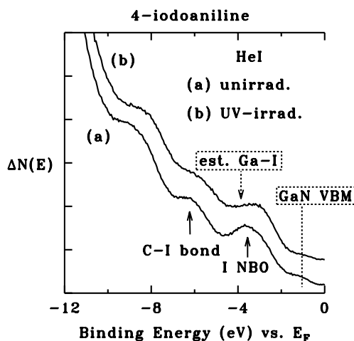
Fig. 8. Similar to Fig. 7a and b but for 4-iodoaniline. Peaks are labelled which derive a large part of their intensity from C–I \sigma -bonding and I NBOs. Also shown is the estimated position of the Ga–I bonding orbital, based on data for \text{I}_2/\text{GaAs}(110) in Ref. [39].
