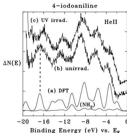
Fig. 6. Similar to Fig. 5 but showing results for 4-iodoaniline.
