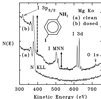
Fig. 2. Mg K \alpha spectra for (a) clean GaN(0001) and (b) after adsorption of 4-iodoaniline. The raw data have been smoothed with a fifth-order, nine-point polynomial. Various Auger and XPS features are labelled. The dashed vertical arrows indicate the N KLL and I MNN Auger peak heights used to quantify changes in I coverage with surface treatment. The instrumental resolution is \sim 1.6 eV. The inset shows the structure of 4-iodoaniline. To clarify notation, the #1 C is bonded to the NH 2 and the #4 to the halogen.
