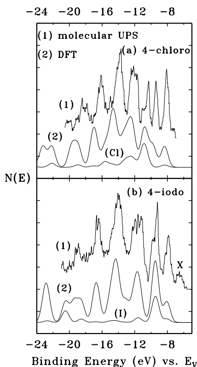
Fig. 4. Comparison of HeII UPS data for gas-phase molecules (Ref. [33], with permission) with DFT results. In either panel, trace (1) gives the data with BE referenced to vacuum, and trace (2) shows the DFT result after alignment at the observed HOMO. Deeper-lying states in the DFT results, below -24 eV, have been truncated. In (b), the feature marked “X” at about -6 eV is apparently an artifact, since it was not assigned in Ref. [33] and not seen in HeI UPS data. The contributions of the respective halogen atoms to the total calculated spectra are shown.
