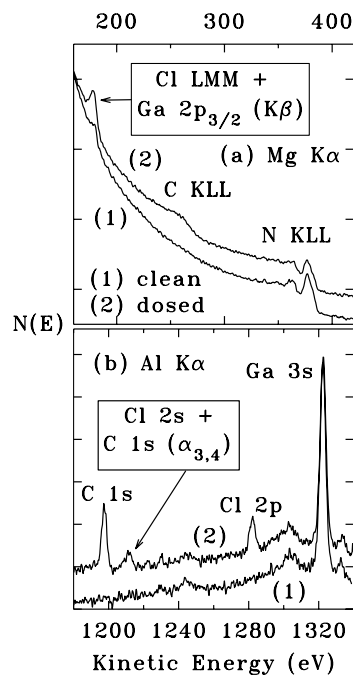
Fig. 1. (a) Partial \text{Mg K}\alpha ( h\nu = 1253.6 eV) spectra for a \text{GaN}(0001) surface before and after a saturation dose of 4-chloroaniline. (b) Partial spectra for \text{Al K}\alpha ( h\nu = 1486.6 eV) excitation, which places features of interest above the range of the strong Ga LMM spectrum. The relative intensities of (a) and (b) are not quantitative, and various XAES and XPS features are labelled. All spectra were recorded with an instrumental resolution of \sim 1.6 eV and smoothed with a fifth-order, nine-point polynomial. The Ga 3s plasmon loss satellite at \sim 1300 eV and the Ga 3s \text{K}\alpha_{3,4} satellite at \sim 1330 eV are not labelled. The very weak feature at \sim 1245 eV is the Ga \text{L}_1\text{M}_{45}\text{M}_{45} XAES peak. Note the different energy scales for (a) and (b).
