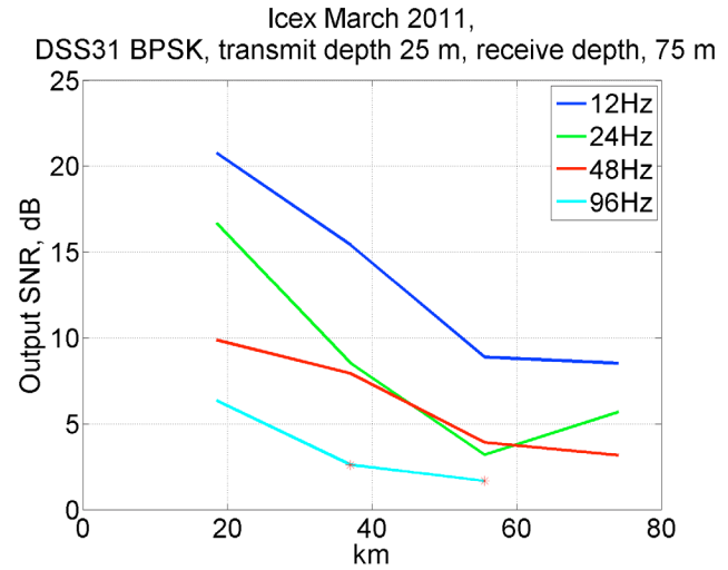
Figure 2. SNR at the output of the adaptive equalizer for the 25m-25m and 25m-75 m transmit-receiver depth cases.
