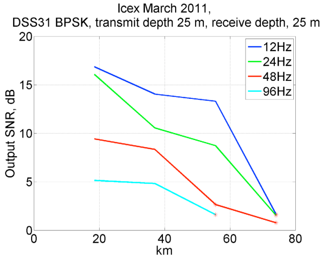
Figure 2. SNR at the output of the adaptive equalizer for the 25m-25m and 25m-75 m transmit-receiver depth cases.
