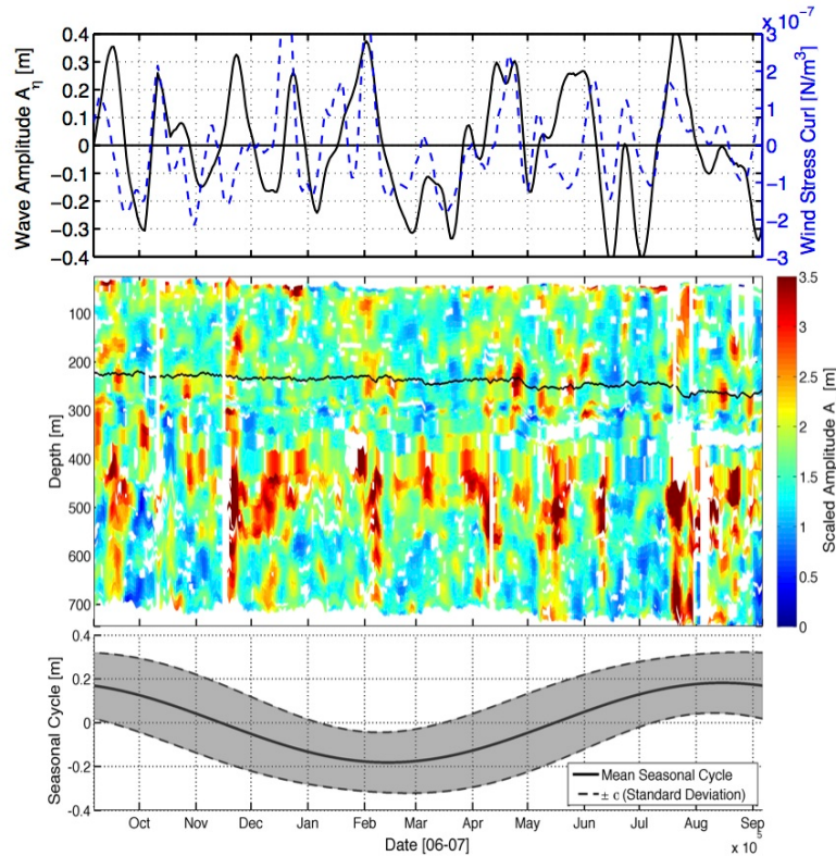
Figure 1: The middle panel shows amplitude of the vertical displacement due to inertial waves (scaled by the square root of the buoyancy frequency to remove the effects of varying stratification) as a function of time and depth. The depth-averaged amplitude in the top 200 m is plotted on the top panel (black line), along with the magnitude of the wind stress curl averaged over a 200km by 200km box around the ITP location for each day (blue). Both fields have been smoothed using a 7-day low-pass filter. The bottom panel shows the depth-averaged seasonal cycle in amplitude, with the dashed lines indicating one standard deviation from the mean.
