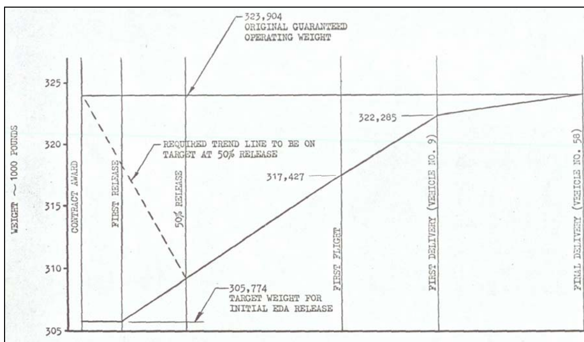
Figure 3-3. Lockheed's Projected Weight Track vs. Phase [11]
