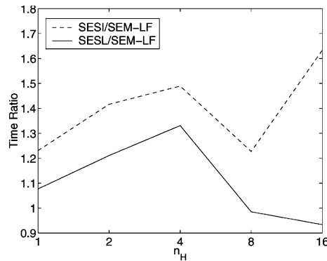
Fig. 18. The ratio of computational cost for SESI/SEM-LF (dashed) and SESL/SEM-LF (solid) for various n_H for Case 5 using N = 8 . The ratios reflect the amount of computer time required to complete a 24 h time-integration.
