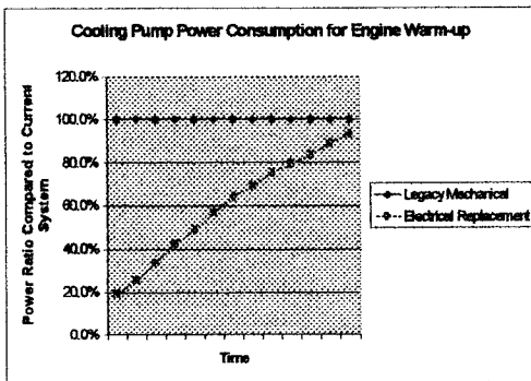
Figure 4 Cooling Pump Power Consumption for Warm-Up
