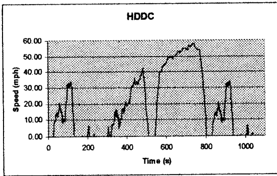
Figure 2. Heavy-Duty Dynamometer Driving Schedule
