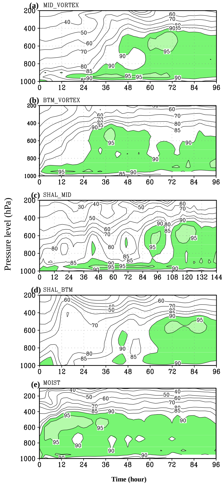
Fig. 9 Time-vertical pressure level (hPa) cross section of RH (%) averaged over a 100 km \times 100km box centered at the MSLP in each experiment. Shading highlights large relative humidity areas that exceed 90%.
