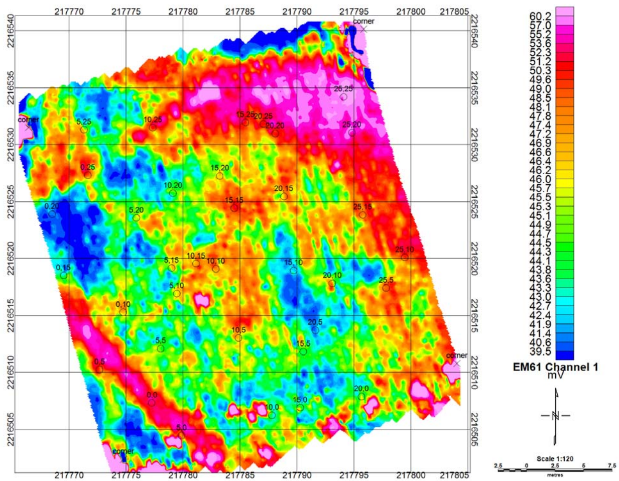
Figure 2.13: EM61 data (Channel 1) collected over the unseeded grid at Waimea. This is the raw data that has only been corrected for position.
