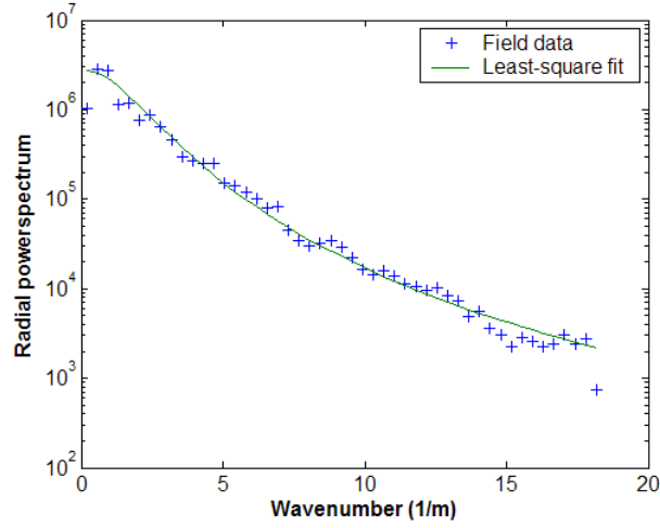
Figure 4.6: Estimated radial power spectrum. The pluses (+) are the radially averaged power spectrum of the EM63 amplitude data, and the solid line is a parametric representation of the radially averaged power spectrum.
