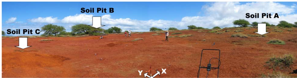
Figure 2.4: Kaho'olawe field site. The top picture shows the location of the soil pits with respect to the 30x30 m grid (outlined in black). Note that soil pit D is located just off the picture. The bottom picture is a panoramic view from the southern corner of the grid.
