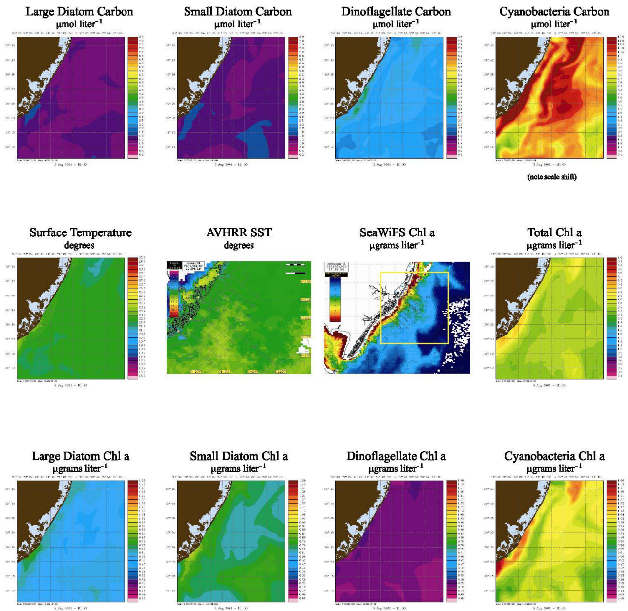
Figure 13: Surface distribution of simulated carbon biomass per functional group (top row); simulated SST, AVHRR SST, SeaWiFS Total Chlorophyll, and simulated Total Chlorophyll (middle row); and simulated chlorophyll a per functional group (bottom row) at the LEO 15 field site August 2 nd during HyCODE 2001 experiment.
