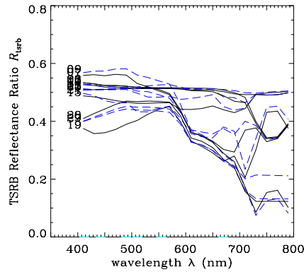
Figure 4. R_{TSRB} under varying depth, bottom types, and IOP conditions.
