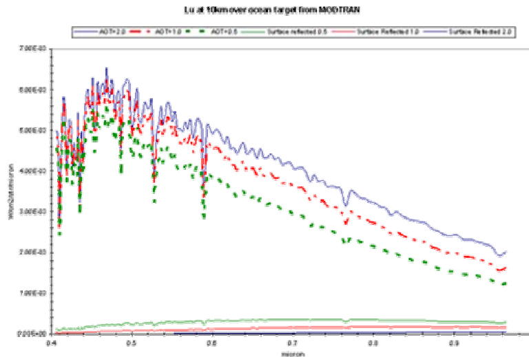
Figure 12. Upwelling radiance at 10 km altitude (upper three curves) for three different \tau_{550} and atmospheric parameters for LEO15 on 7/31/2001 as modeled by MODTRAN4. Lower three curves are the radiance reflected from the default ocean surface in the model.
