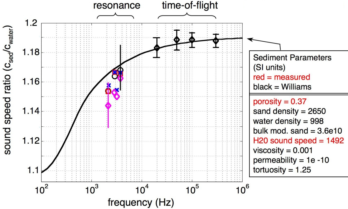
Fig. 6. Normalized sound speed measurements, the result of new analysis, are compared to the EDFM (solid line). Black circles and red squares were obtained at two different sediment locations, with the sound source in center, and hence were inferred from the resonance frequencies of axisymmetric modes. Blue x's and magenta diamonds were obtained at the same two sediment locations, but with the sound source located off-center, and hence were inferred from the resonance frequencies of asymmetric modes. Black diamonds are from the time-of-flight measurements. Error bars represent length and time uncertainties, but due to the close grouping of some of the data, they are not shown for every data point. The material parameters (in pure SI units) required for evaluation of the EDFM are shown in the table to the left of the plot. The values shown in red were measured and specifically refer to the sediment in this study. The values shown in black were taken from Ref. [10], for a similar type of sand. No adjustment of material parameters was conducted, nor was any fitting performed. The EDFM agrees very well with the time-of-flight measurements, within the range of measurement uncertainty in each case. The upper third of the resonance-based measurements are in agreement with the EDFM, but the degree of agreement diminishes as frequency continues down. For the lowest few frequencies, the data points and the upper limit of the error bars are over-predicted by the EDFM.
