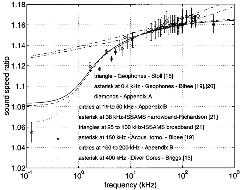
Fig. 1-a. State-of-the-art model/data comparison for the sound speed in a sandy water-saturated sediment. The citations in the legend refer to those in Ref. [26]. The theoretical curves are: solid line=Biot/Stoll [9]; dashed line=Williams [10], dash-dot lines=Buckingham's model for two values of fluid viscosity [8]; dotted line=best fit Biot/Stoll model for input parameters outside of measured values. Note the scarcity of data from the low-kHz and below. Also note that the Biot and Williams models do a better job of predicting the data than the Buckingham model does. (Figure adapted from [26].)
