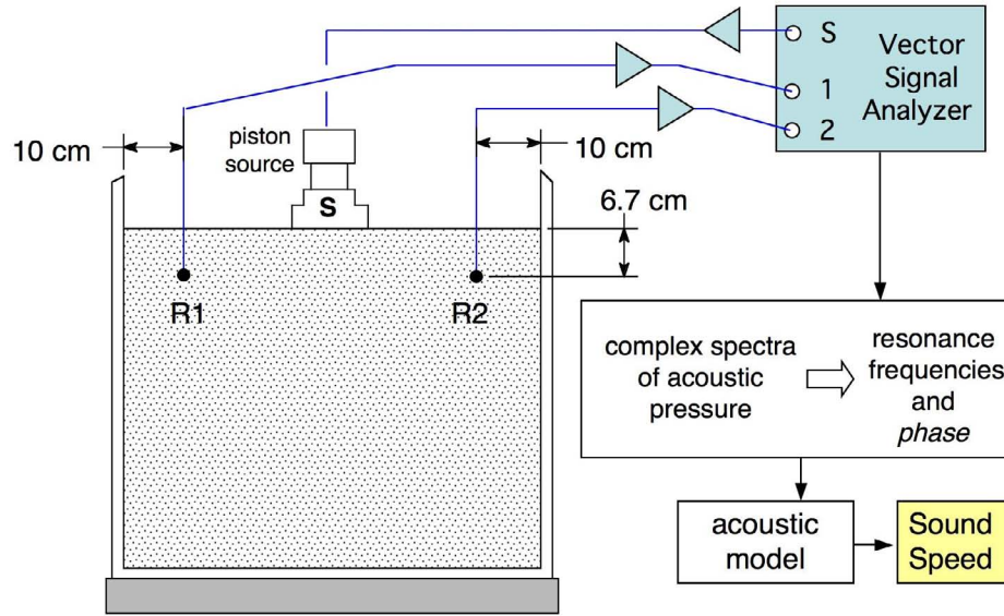
Fig. 5. A schematic diagram of the resonance experiment is shown. A constant-velocity tonpiltz source was used to excite the system. By placing it in the center, symmetric modes were excited. By placing the source midway between the center and the wall, asymmetric modes were excited. The source was driven with periodic chirps and the pressure spectra were recorded at positions R1 and R2. Analysis of the spectra yielded resonance frequencies which were in turn related to the frequency-dependent sound speed of the sediment. The effect of the finite impedance of the tank walls was accounted for, and found to be small.
