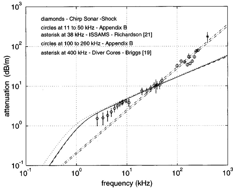
Fig. 1-b. Same as Fig. 1-a, except for attenuation. Note that here, the Buckingham model does a better job of predicting the data than the Biot and Williams models do. (Figure adapted from [26].) Also note that there is attenuation data below about 3 kHz.
