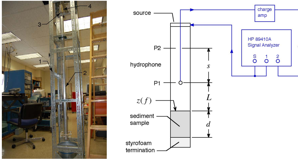
Fig. 2. On the left is shown a photograph of part of the impedance tube system in our laboratory, including the supporting framework (1), the impedance tube (2), the hydrophone (3), and the hydrophone positioning system (4). The tube in the picture is a temporary place holder for the heavy-walled tube, while it undergoes machine shop operations. On the right is a schematic diagram of the impedance tube system.
