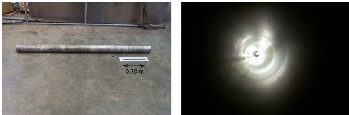
Fig. 3. On the left is shown a photograph of the heavy-walled impedance tube during machine shop operations. The 0.30 m length machinist's rule indicates the size of the tube, which is 1.83 m in length. On the right, the view down the center of the tube is shown, illuminated from the far end with a flashlight, after gun drilling and honing. Note the smoothness of the inner tube wall.
