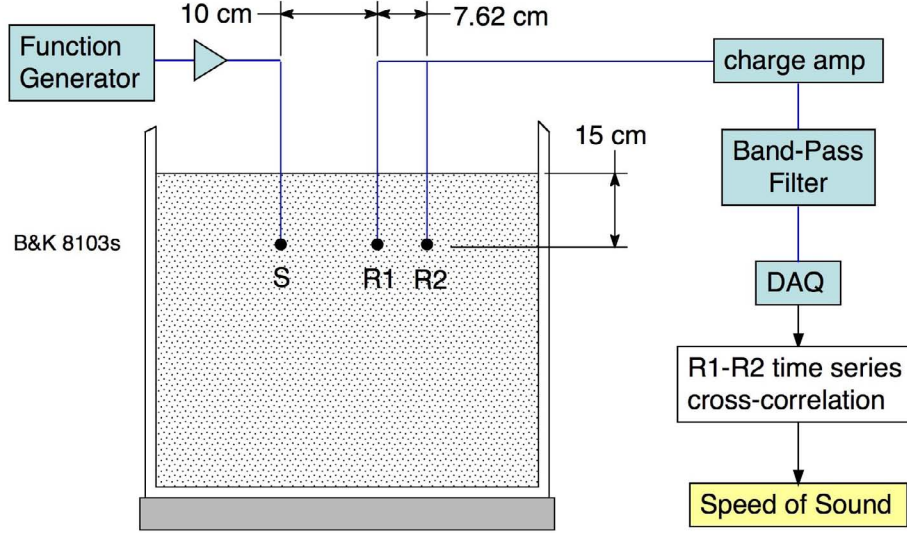
Fig. 4. A schematic diagram of the time-of-flight experiment is shown. A large thin-walled cylindrical container was filled with 60°C degassed water and sorted and washed medium grain blasting sand. Three B&K 8103 hydrophones were placed in the sediment and time-of-flight measurements were obtained after cooling. A function generator and power amplifier were used to drive one of the 8103s as a source. The remaining two 8103s were used as receivers. Their signals were conditioned with a charge amp and a band-pass filter. The voltage signals were acquired with a digital oscilloscope and cross correlated to extract the time-of-flight. Sound speed was then calculated from the 7.62 cm sensor separation distance.
