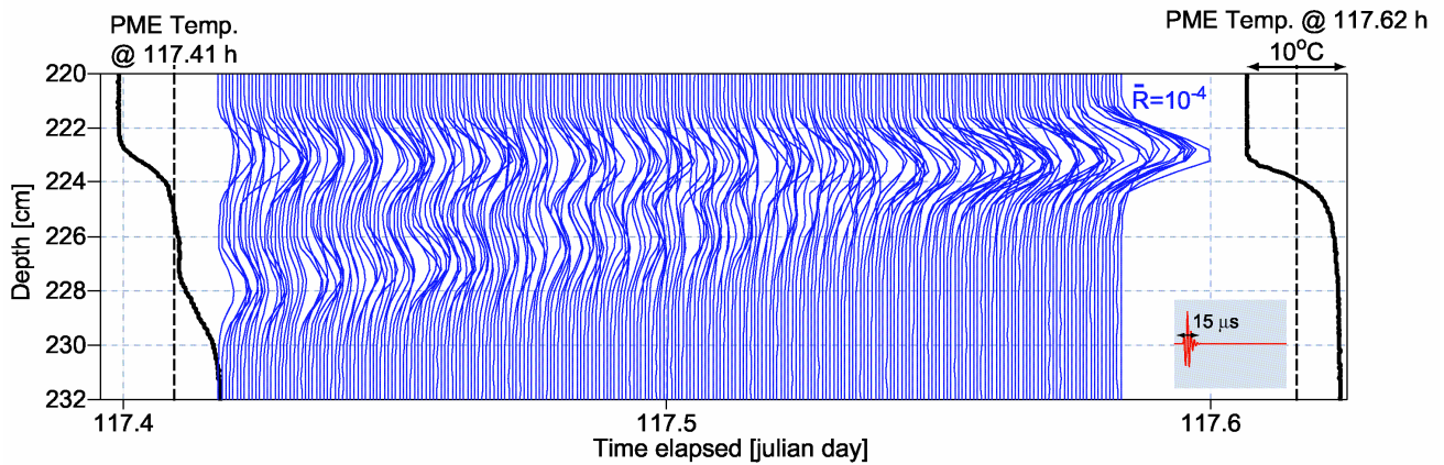
Figure 7. Using high-frequency broadband acoustic scattering returns it is possible to observe the evolution and dynamics of multiple double-diffusive interfaces. Shown here is the merging of two double-diffusive steps ( P_{scat}/P_{inc} ) as a function of time and depth. A 15 \mu s long chirp, 200-300 kHz, was used. Temperature profiles (black lines) obtained with the microstructure instruments are shown to the left and right of the acoustic data.
