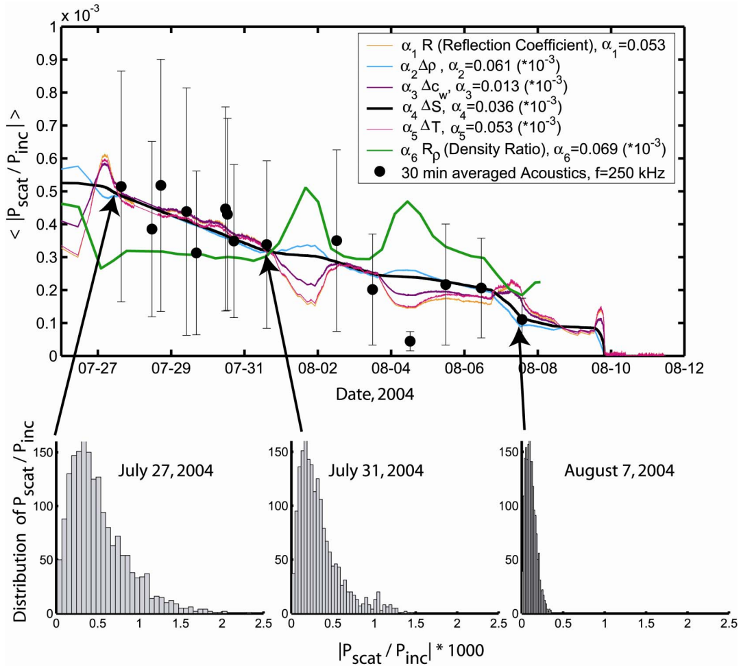
Figure 5. Mean amplitude of P_{scat}/P_{inc} at 250 kHz (black circles, error bars represent a standard deviation) during the July and August, 2004, experiment. The averages were only performed for acoustic data files that were at least 30 minutes in duration, to assure that multiple intermittent scattering events were probed during each data acquisition period. A least-squared fit was performed to obtain the best fit scaling parameter \alpha_{1-6} between the mean P_{scat}/P_{inc} at 250 kHz and the following parameters: the reflection coefficient, R (orange line), density step, \Delta\rho (blue line), sound speed step, \Delta c_w (purple line), salinity step, \Delta S (black line), temperature step, \Delta T (pink line), and density ratio, R_\rho (green line), as calculated from the CT sensors in the upper and lower mixed-layers were. The resulting scaling parameters are shown in the legend. The best fit was obtained for the difference in the salinity between the upper and lower mixed layers. The histograms show the distribution of the amplitude of P_{scat}/P_{inc} at 250 kHz for three individual 30 minute long data acquisition periods.
