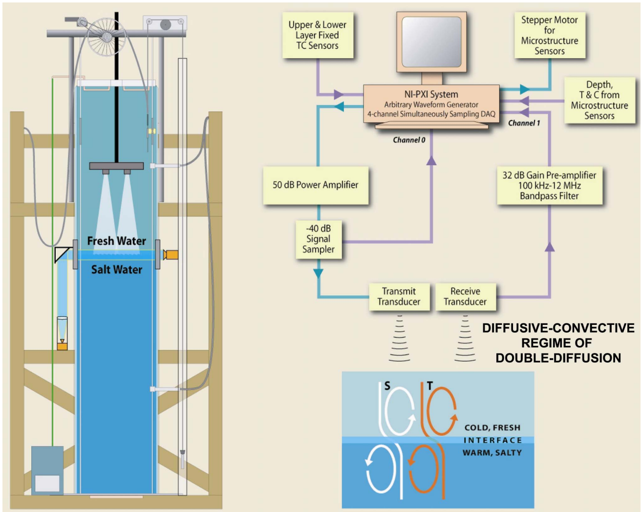
Figure 1. Schematic showing the laboratory constructed for measuring high-frequency broadband (200-300 kHz and 350-650 kHz) acoustic scattering from the diffusive regime of double diffusion. The lower mixed-layer is filled with warm, salty (and dense) water, and the upper layer is filled with cold, fresh water: a sharp interface separates the mixed layers. A shadowgraph system was built to obtain optical images of the interface, and small-scale temperature and conductivity measurements were performed using a fast-response thermistor and four-electrode conductivity probe. The tank is approximately 4.6 meters deep and 1 meter wide. Two fixed temperature and conductivity sensors are mounted in the upper and lower mixed-layers, providing continuous monitoring on the mixed layer properties. A box diagram of the data acquisition system used to collect the acoustic and ancillary data is shown.
