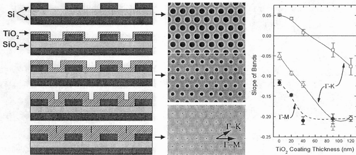
Figure 25. Schematic cross-section of the 2D triangular lattice illustrating the progressive coating of \text{TiO}_2 onto the lattice. The conformal deposition by ALD yields equal growth at the bottom and sides of the air holes as well as the top surface of the slab. For full \text{TiO}_2 infiltration, the air holes are completely filled, creating a \text{TiO}_2 cladding layer. The SEM images show the top surface of the uncoated sample and after coating with 40 nm and 120 nm of \text{TiO}_2 . The right panel shows the measured slopes of several bands that are observed to decrease with increasing \text{TiO}_2 coating thickness.
