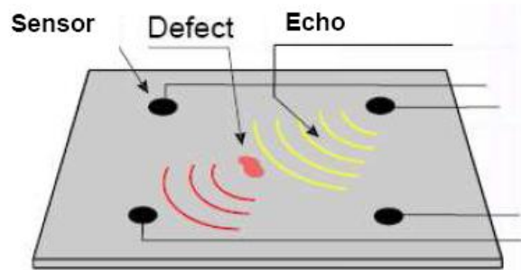
Figure 2.5-2 Acousto Ultrasonic (Pitch-Catch) Principle
