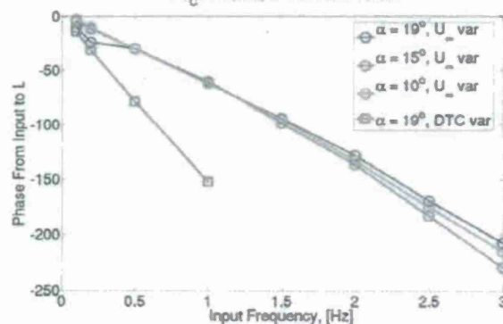
Figure 7. Experimental phase lag in lift response of a semi-circular wingplan to incoming flow velocity variation, and to harmonically modulated duty actuation duty ratio, in open loop.
