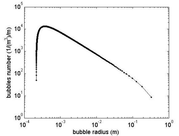
Figure 2. Estimated bubble size distribution after the initial break-up of the explosion bubble.
