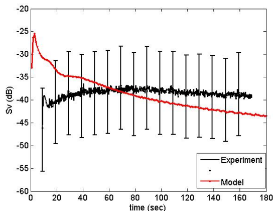
Figure 9. Backscattering cross-section at the horizontal slice of the rising bubble cloud. Depth of the slice location is 3 feet.
