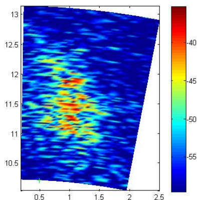
Figure 8. Backscattering cross-section per unit volume calculated from sonar data in a horizontal slice through the bubble cloud.
