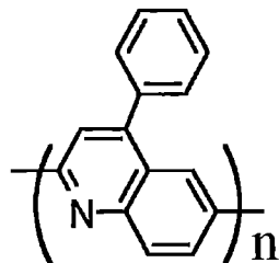
PPQ: poly(2,6-(4-phenylquinoline))
