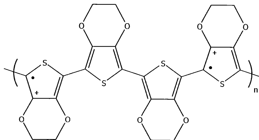
PEDOT Poly(3,4-ethylenedioxythiophene)
