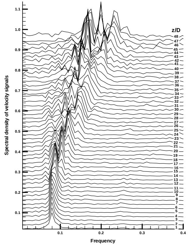
Figure 2. Frequency spectra of crossflow velocity for run 3.
