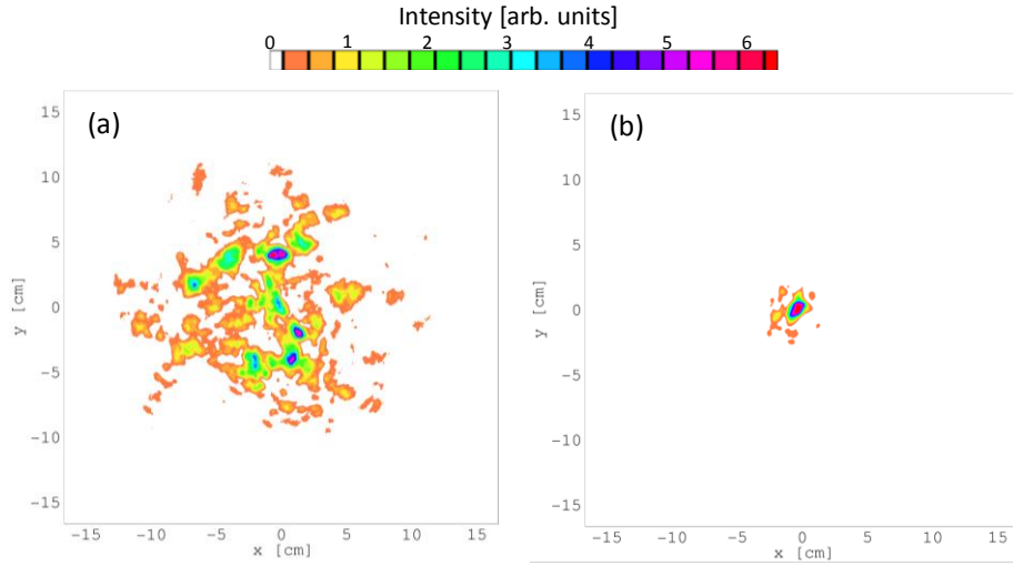
Figure 5: Intensity profiles of a beacon beam on the target after one pass. An intensity gain factor of 8 is assumed in the phase conjugating cell and Rytov variance \sigma_R^2 = 2 . In the absence of turbulence, the illuminator system produces a spot size of 1 cm on the target.
