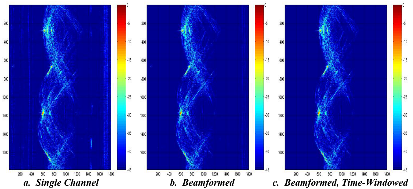
Figure 1. Example Waterfall Plots of Target Impulse Response Function [Echo amplitude is color coded; the vertical axis is ping number (aspect angle), the horizontal axis is sample number (time)]
