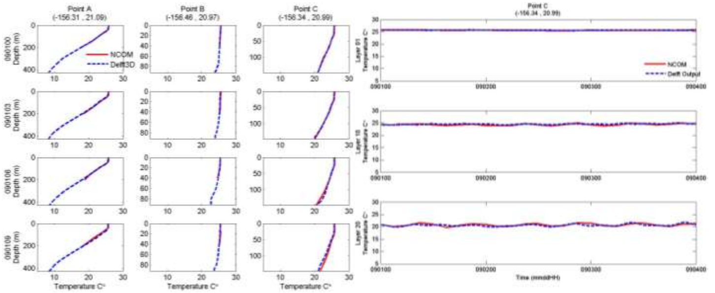
Figure 10. Left: Profile comparisons of temperature at Points A (left), B (middle), and C (right) in the Maui domain. The top row shows results from the beginning of the model runs. Model time increase as you move down the rows. Delft3D (blue dash) and NCOM (red line) results are shown. Right: Time series comparisons of temperature at Point C in the Maui domain. The top shows a near surface comparison; the middle shows a mid-depth comparison, and the bottom shows a near bottom comparison. Delft3D (red dash) and NCOM (blue line) results are shown.
