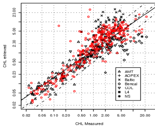
Figures 5. Shows the regressions of case 1 Chlorophyll retrieved from the model or by the NASA OC4V4 algorithm against Chlorophyll measured in situ in both case 1 and case 2 waters. Most notable is the result that RMS error is reduced for the IOP model by over an order of magnitude and the bias is halved.
