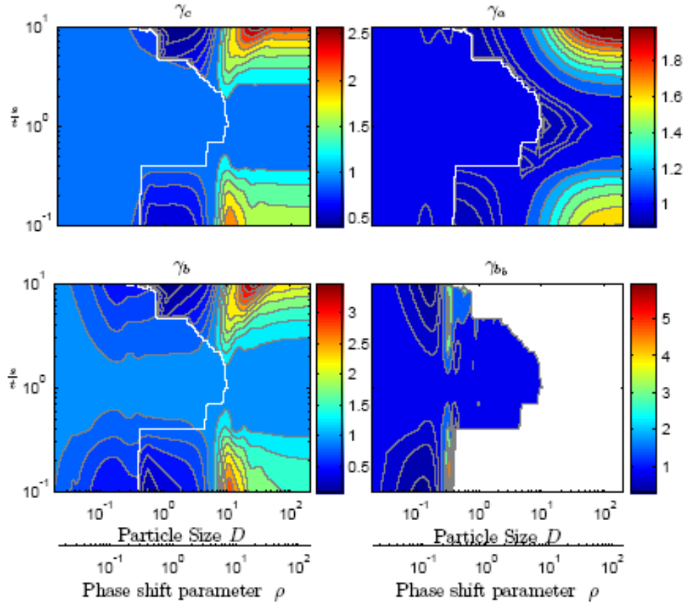
Figure 3. Bias (ratio of optical property for a spheroid relative to a sphere with the same volume) as function of size, and axis ratio (t/s axis of symmetry vs. the other axis) for attenuation (top left) absorption (top right), scattering (bottom left) and backscattering (bottom right) for a phytoplankton like particle with index of refraction n=1.05+0.01i .
